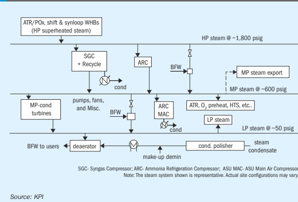
Fig. 4: Steam system of a next generation ATR-based ammonia plant
