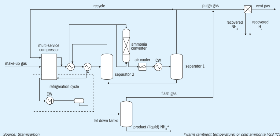
Fig. 2: NX STAMI™ Ammonia high-pressure design process diagram
