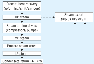
Fig. 1: Conventional steam-rich utility architecture common to ammonia, and methanol plants
