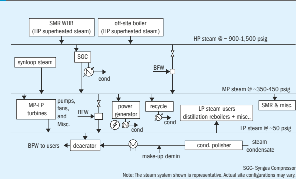
Fig. 5: Steam system of a conventional methanol plant (SMR only)
