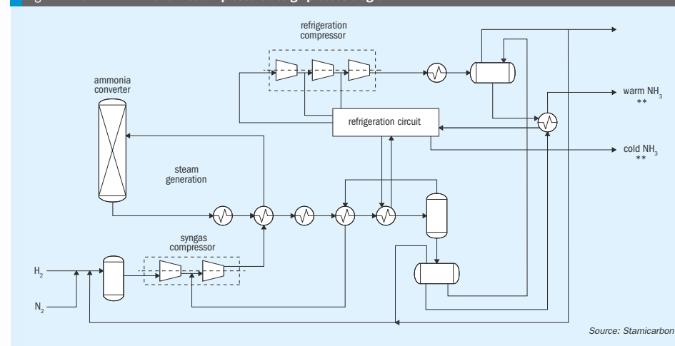
Fig. 1: NX STAMI™ Ammonia medium-pressure design process diagram
