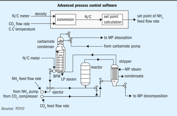
Fig. 2: Concept of advanced process control (APC) for urea plant operation
