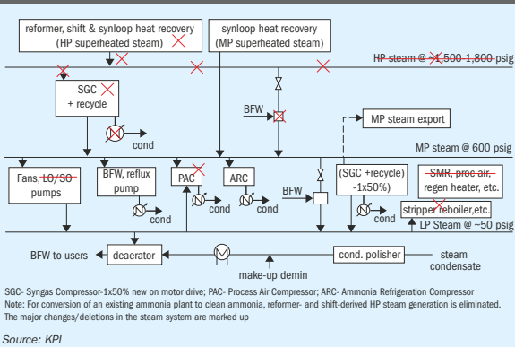
Fig. 3: Steam system with conversion to a clean ammonia plant
