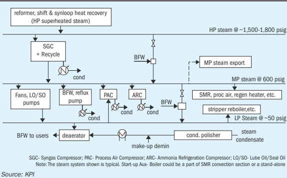
Fig. 2: Steam system for a conventional ammonia plant
