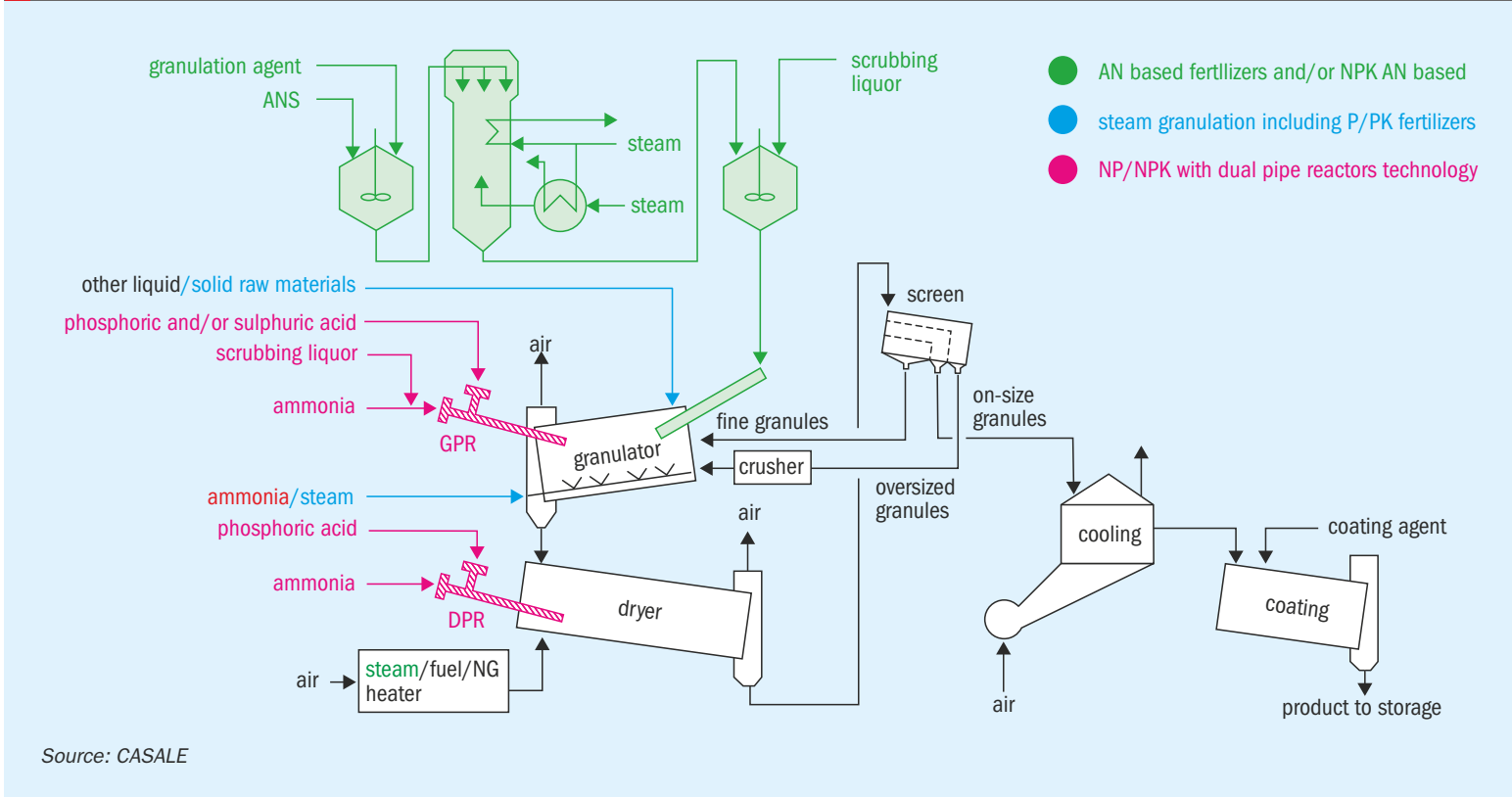
Fig. 3: An integrated granulation plant incorporating three different CASALE processes, including dual pipe reactor technology
