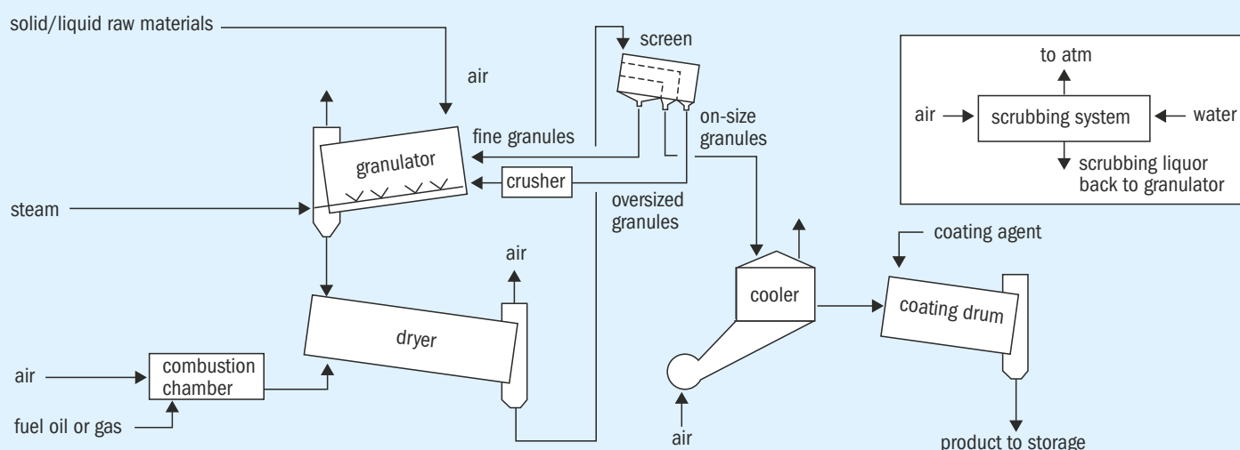
Fig. 2: CASALE's steam granulation process
