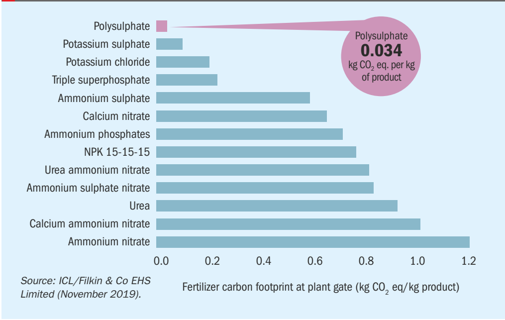
Fig. 1: The carbon footprint of Polysulphate in comparison to other commonly-used fertilizers
