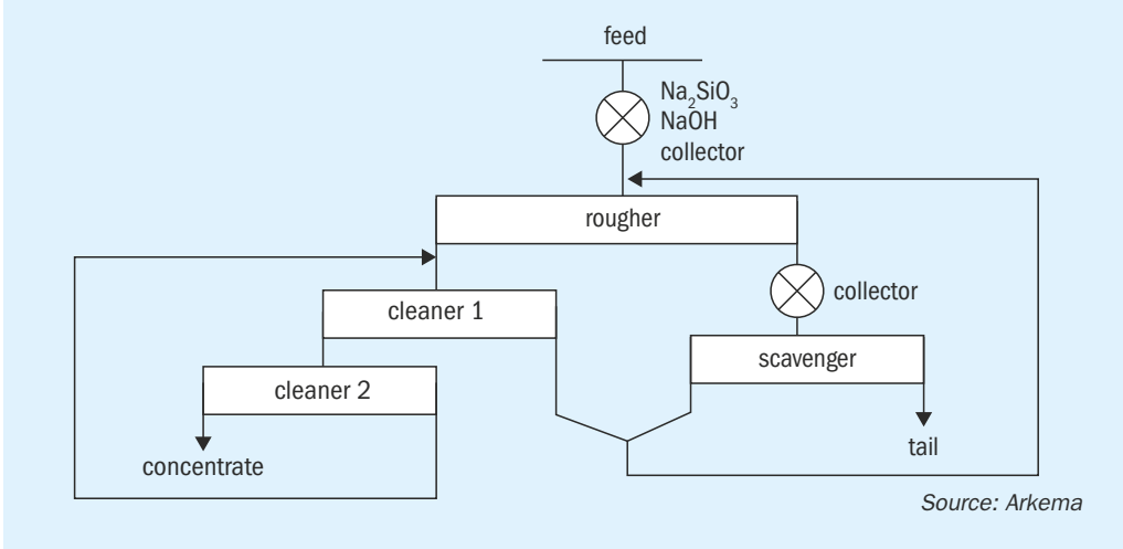
Fig. 4: Process schematic for a locked-cycle flotation test (five cycles) with 400 g/t of CustoFloat® M collector
