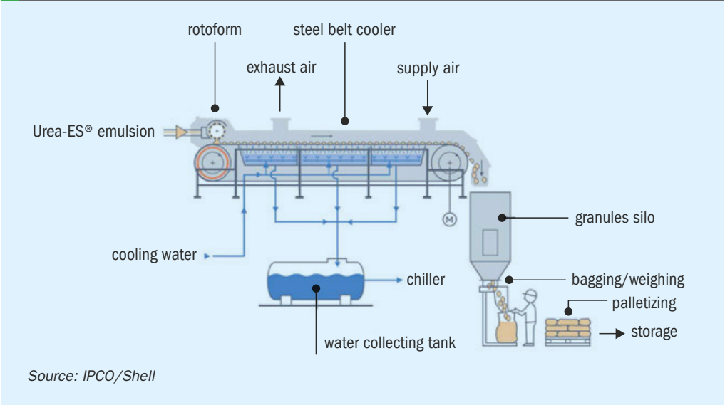
Fig. 2: IPCO Rotoform pastillation process for Urea-ES®
