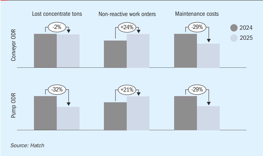
Fig. 5: Conveyor and pump operator driven reliability impacts
