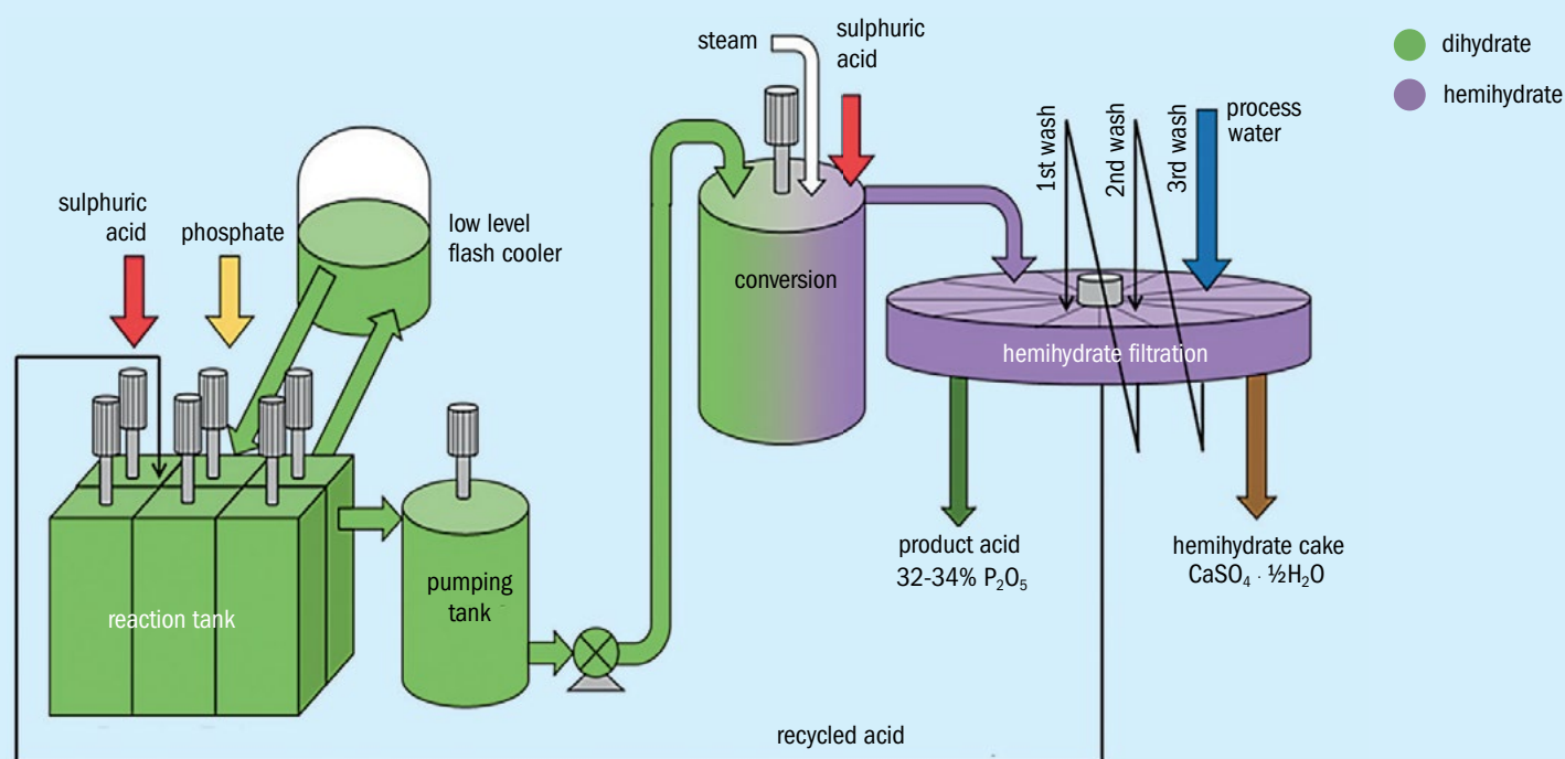
Fig. 2: Prayon's DA-HF process: this solution can provide a dry, low- P_2O_5 gypsum product from most phosphate rock types on the market
