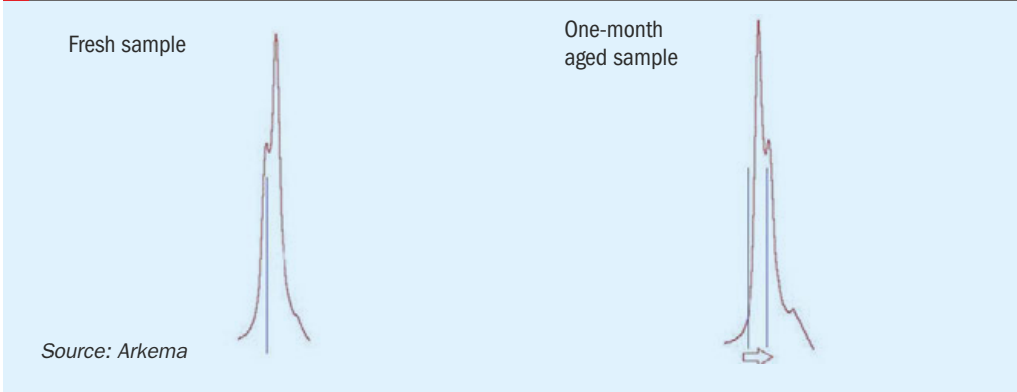
Fig. 2: CustoFloat O (experimental version): analysis spectra showing esterification after one month
