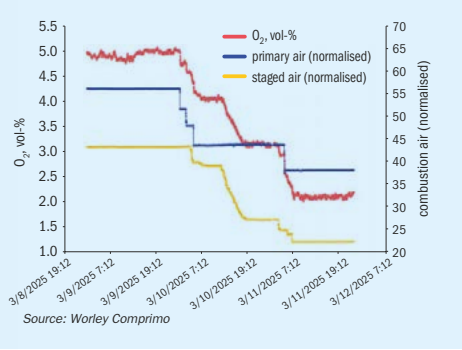
Fig. 8: Incinerator primary and staged air flows and flue gas oxygen concentration in SRU-1
