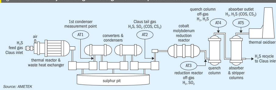
Fig. 1: SRU and TGTU layout. The tags AT1 through AT5 indicate potential measurement locations in the SRU and TGTU
