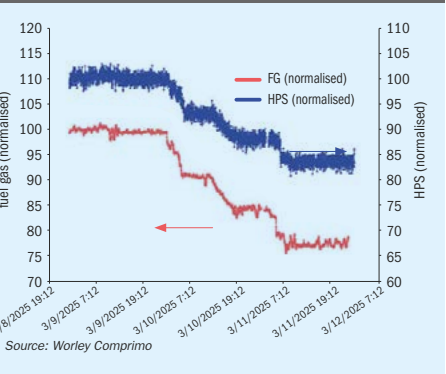
Fig. 7: Incinerator fuel gas consumption and WHB high-pressure steam production in SRU-1
