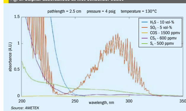
Fig. 2: Sulphur absorbances at first condenser outlet
