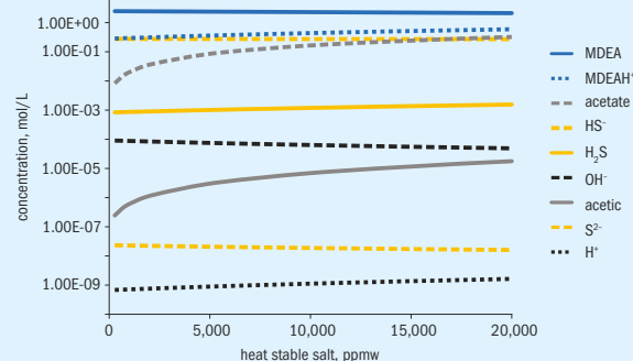
Fig. 2: Speciation of 0.1 mol/mol loaded MDEA solution with increasing heat stable salts (acetate)
