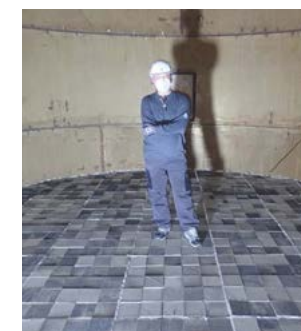
Fig. 3: PPH catalyst hurdle equipped with P&P's VividOx catalyst.
