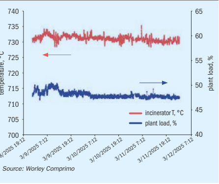
Fig. 9: Incinerator temperature and plant load in SRU-1
