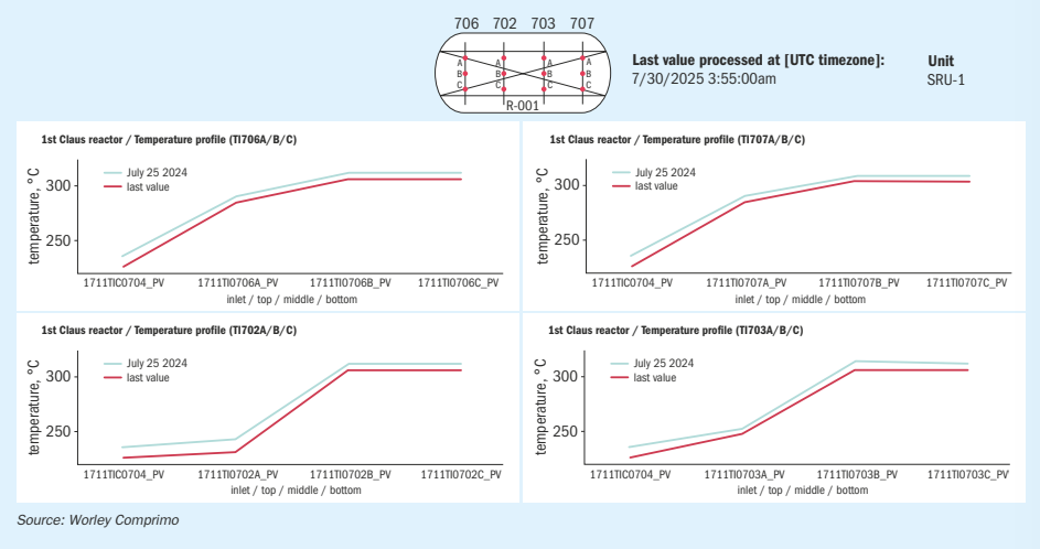
Fig. 3: Comprimo Insight dashboard with temperature profile across the 1st Claus reactor catalyst bed for plant SRU-1, actual values compared to fresh catalyst
