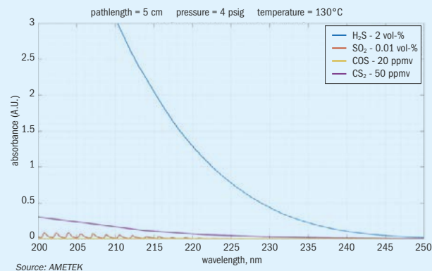
Fig. 5: Sulphur absorbances at TGTU absorber outlet
