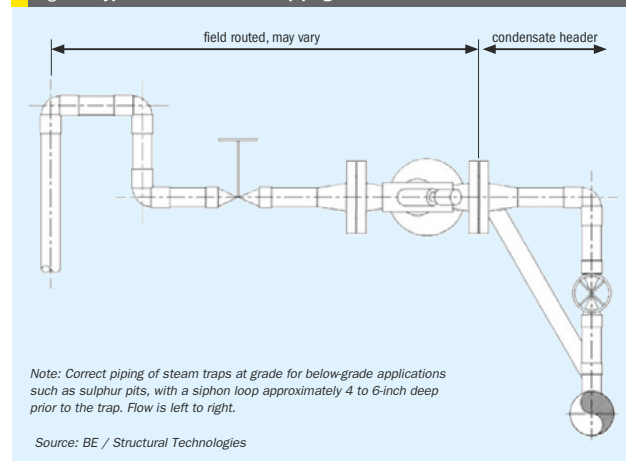
Fig. 10: Typical condensate return piping
