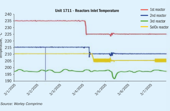
Fig. 5: Adjustment for RITs for 1st, 2nd Claus reactors and SelOx reactor for SRU-1. Data collected between 01 March (00:00) - 07 March 2025 (23:59)
