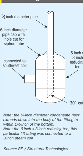
Fig. 8: A cross-section diagram of a lift fitting
