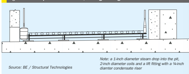
Fig. 7: An example of a steam coil, flowing from right to left
