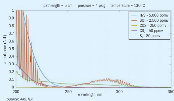
Fig. 4: Sulphur absorbances at quench tower inlet
