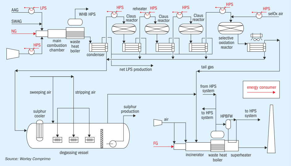
Fig. 4: Typical process flow diagram of an SRU featuring a 3 Claus + 1 SelOx reactor configuration, indicating major energy-consuming equipment
