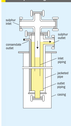
Fig. 4: Diagram of a conventional sulphur seal leg
