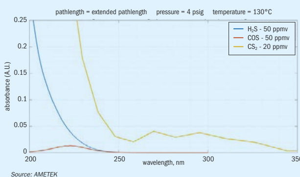
Fig. 5: Sulphur absorbances at TGTU absorber outlet
