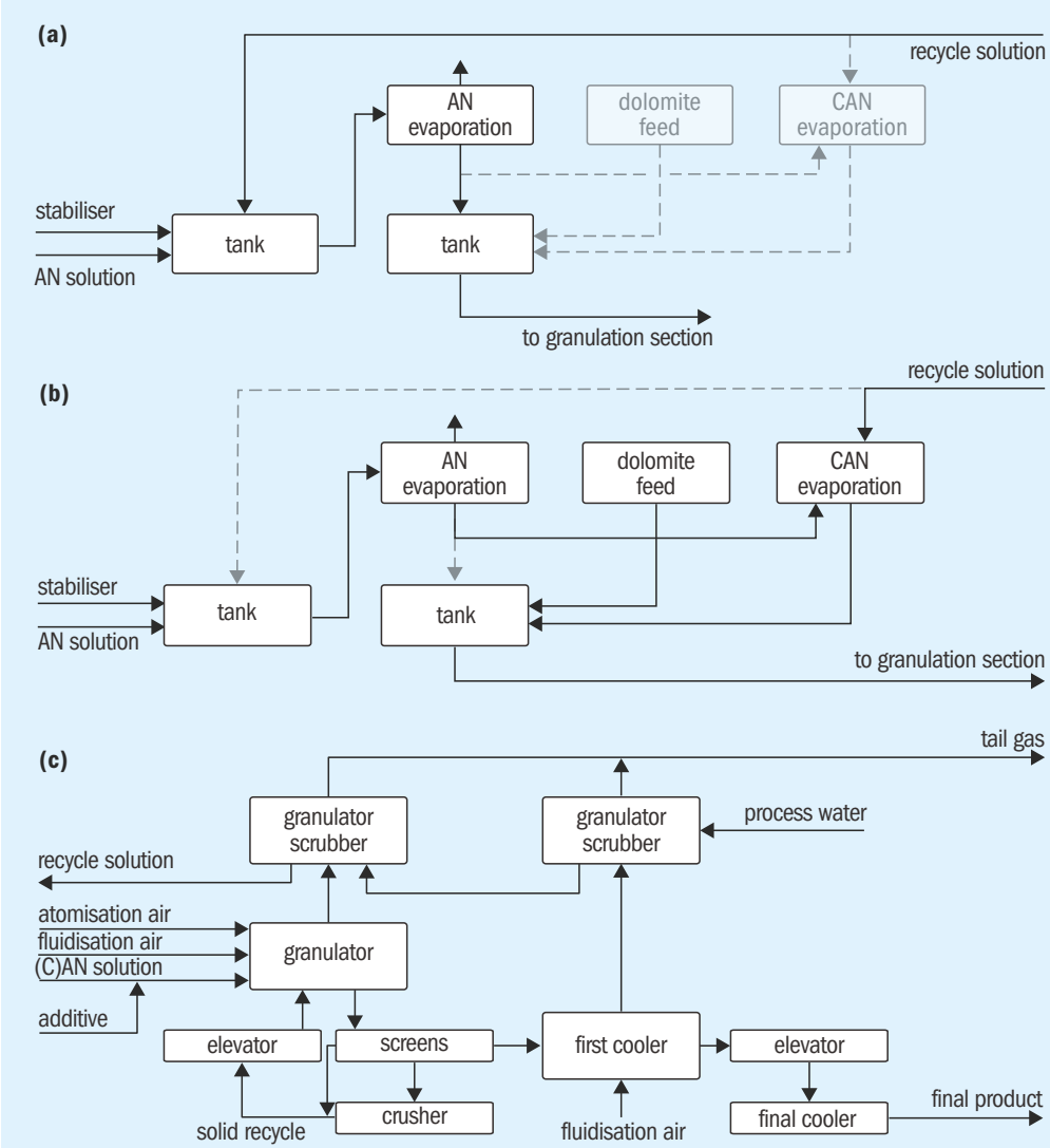
Fig. 4: Fluidised bed granulation: (a) AN preparation loop, (b) CAN preparation loop, (c) AN/CAN granulation section
