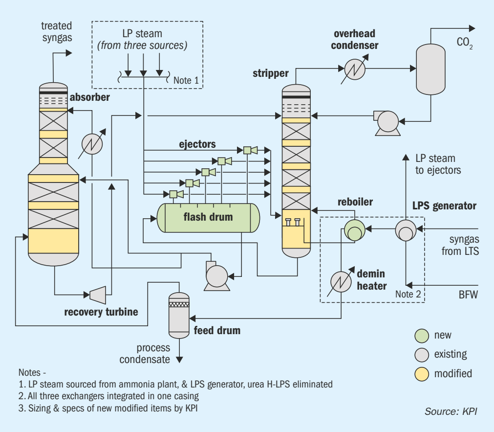
Fig. 9: Post-revamp Benfield system
