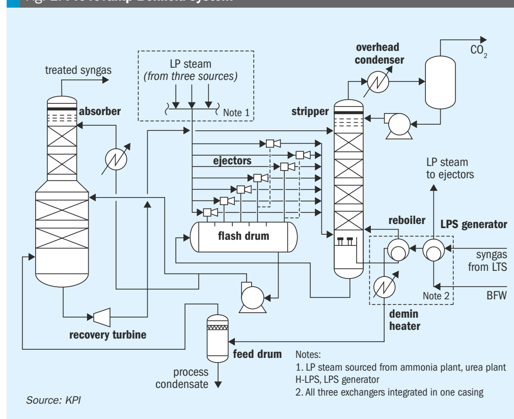
Fig. 1: Pre-revamp Benfield system
