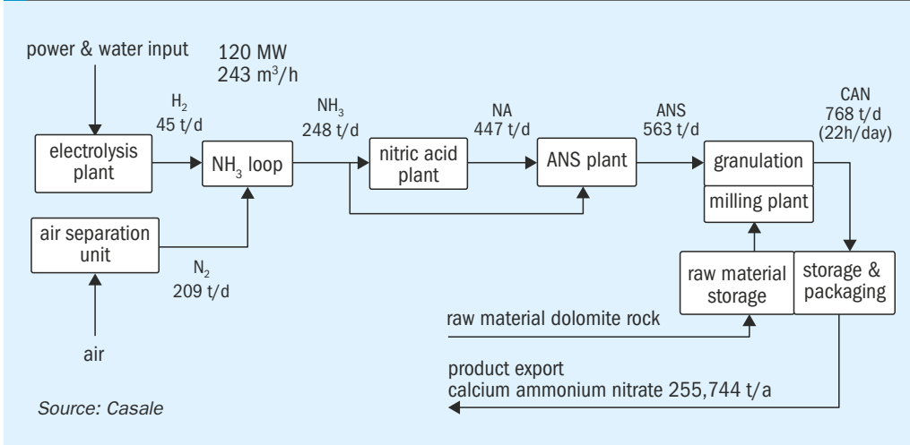
Fig.6: Technology applied in the Villeta Green Fertilizer Project in Paraguay
