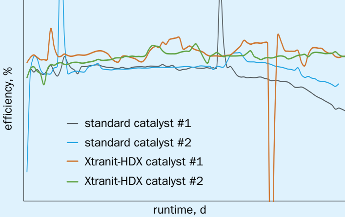
Fig. 6: Comparison of standard catalyst packages versus Umicore’s Xtranit-HDX catalyst gauzes
