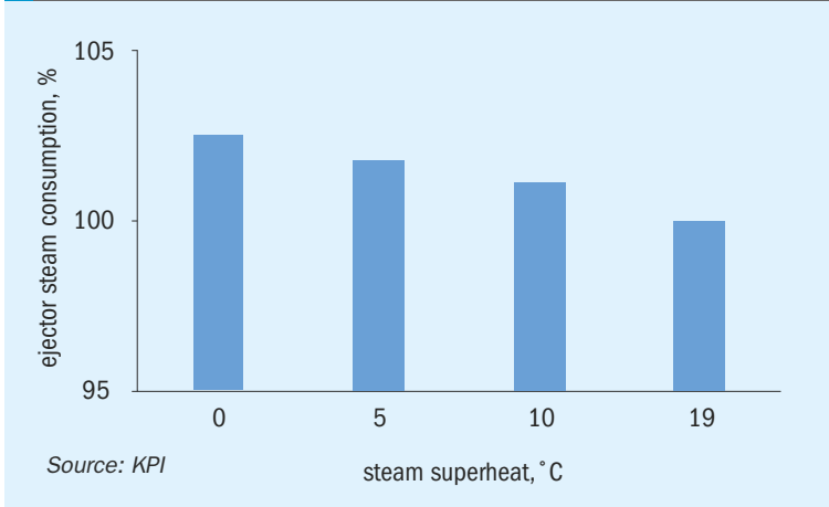
Fig. 7: Ejector steam consumption – impact of steam superheat
