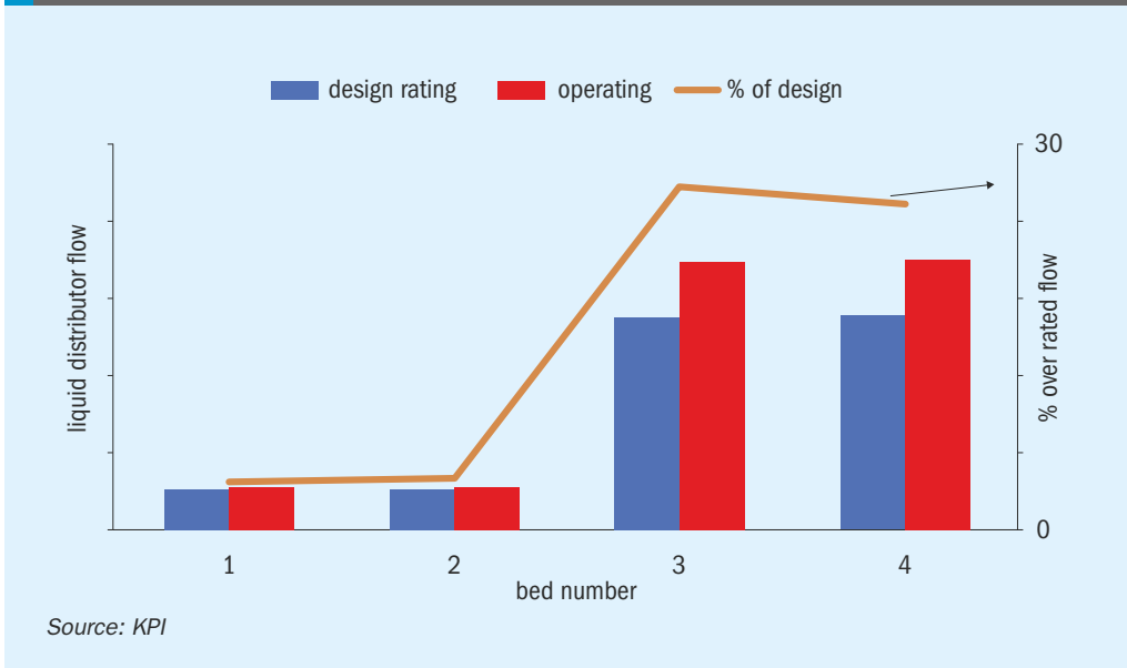
Fig. 4: Absorber liquid distributors – rated vs actual flowrate
