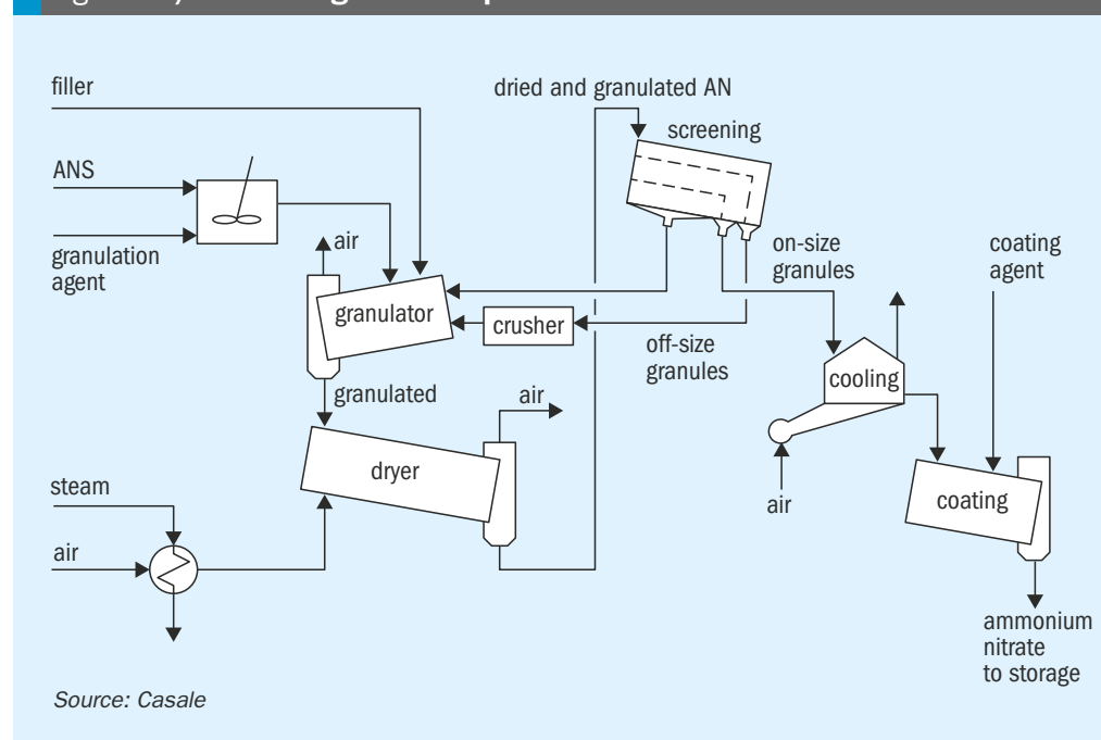
Fig. 5: AN/CAN drum granulation plant
