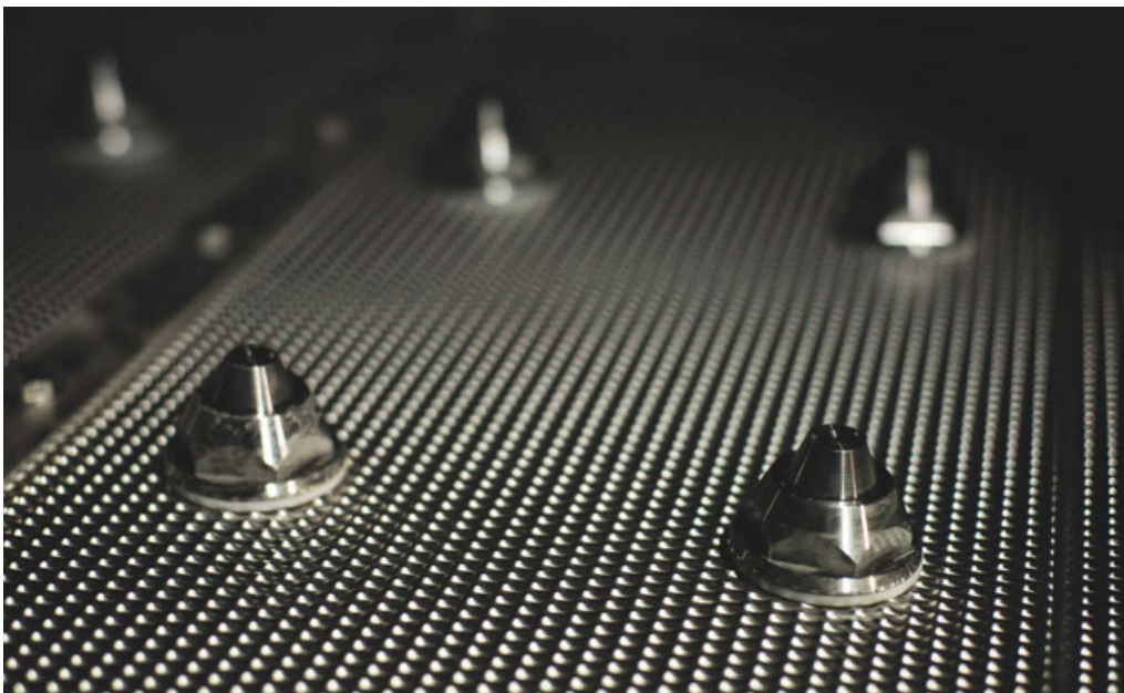
Fig. 2: Granulator film spraying nozzles.
