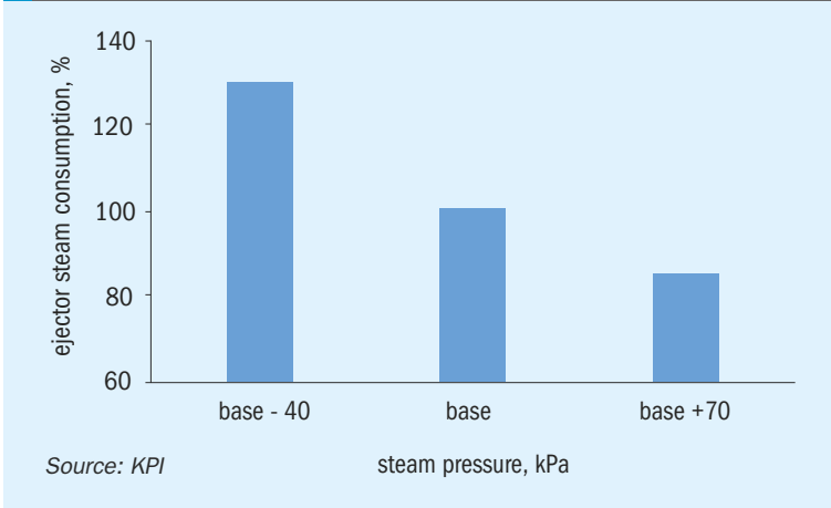
Fig. 8: Ejector steam consumption – impact of steam pressure
