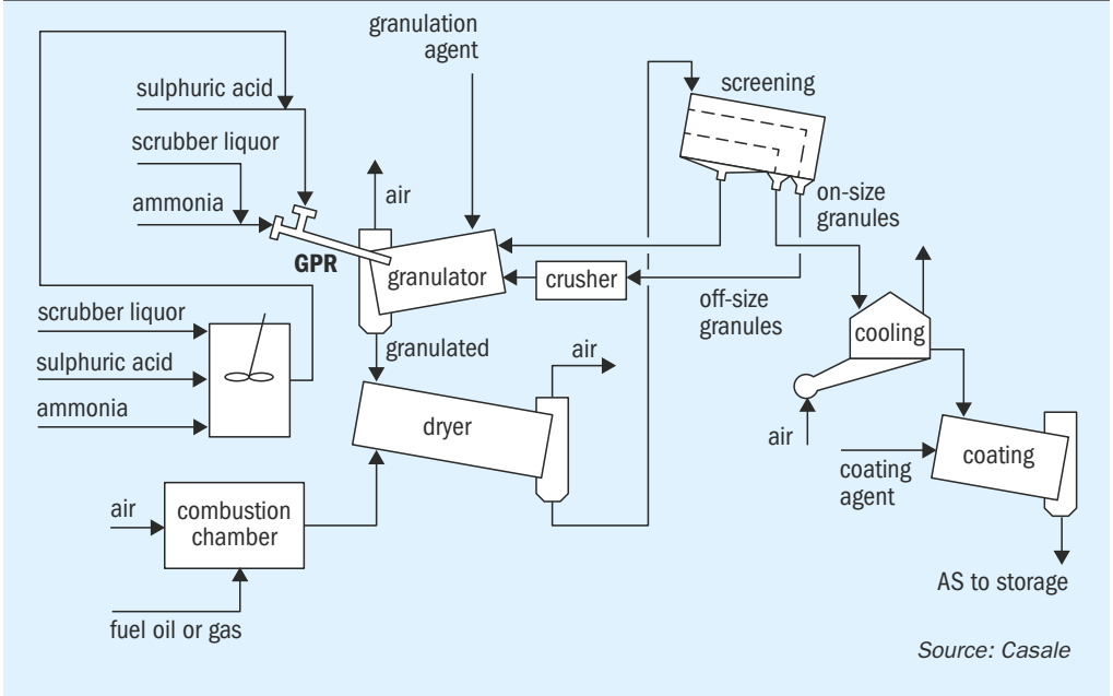
Fig. 7: AS drum granulation plant
