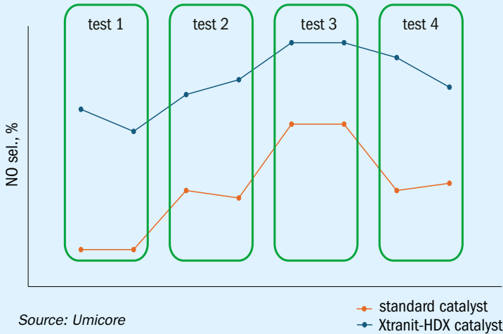
Fig. 5: Pilot plant tests at high pressure conditions with varying plant load (32-64 tN/m 2 /d)
