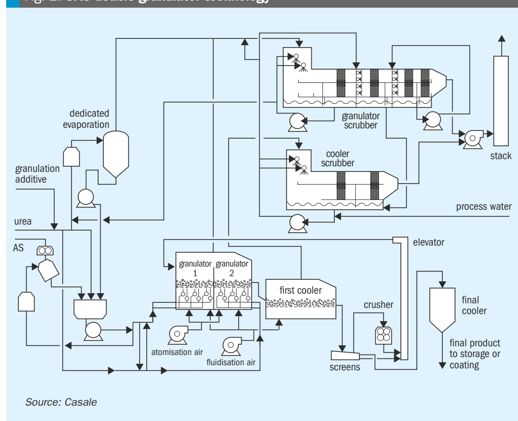
Fig. 2: UAS double granulator technology
