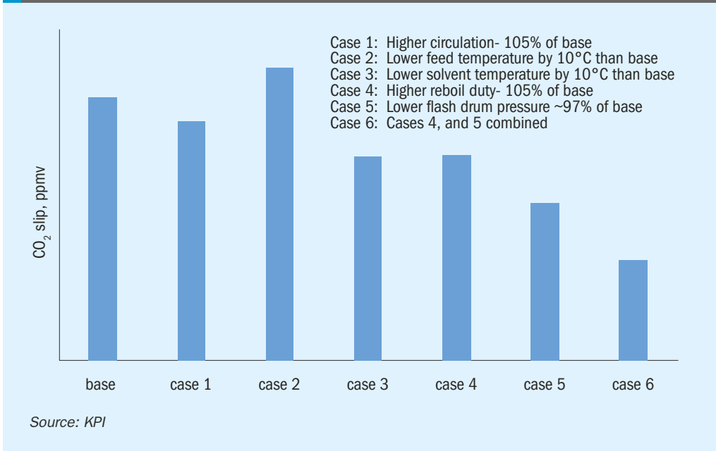
Fig. 2: CO 2 slippage – sensitivity of various parameters
