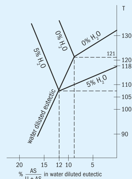
Fig. 1: Urea – AS eutecticum graph
