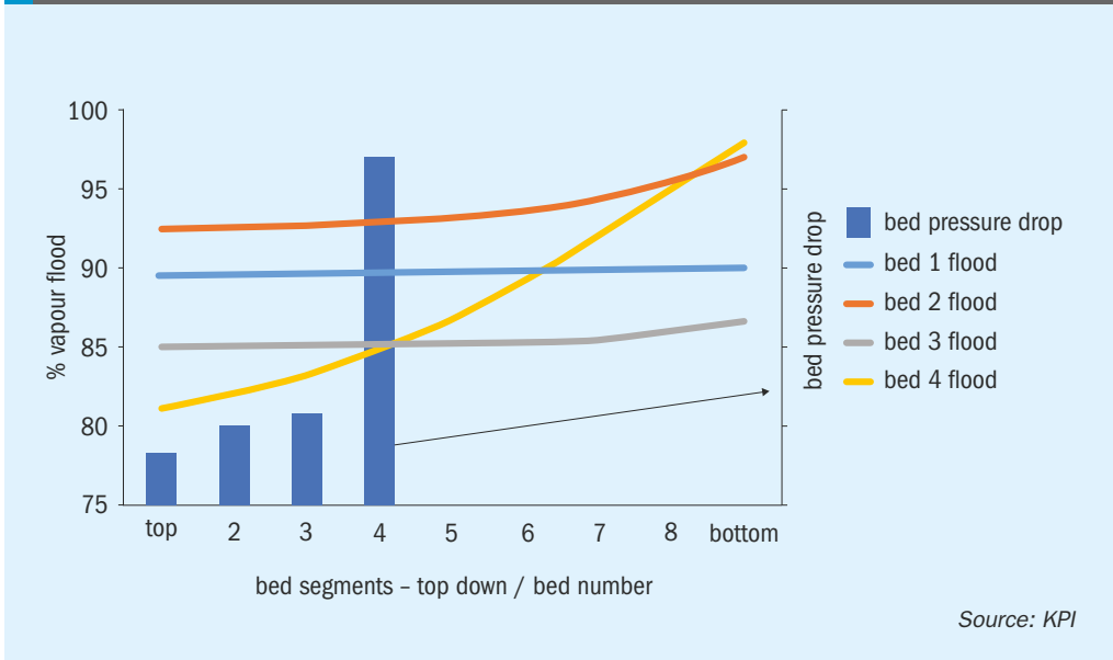
Fig. 3: Absorber bed hydraulics
