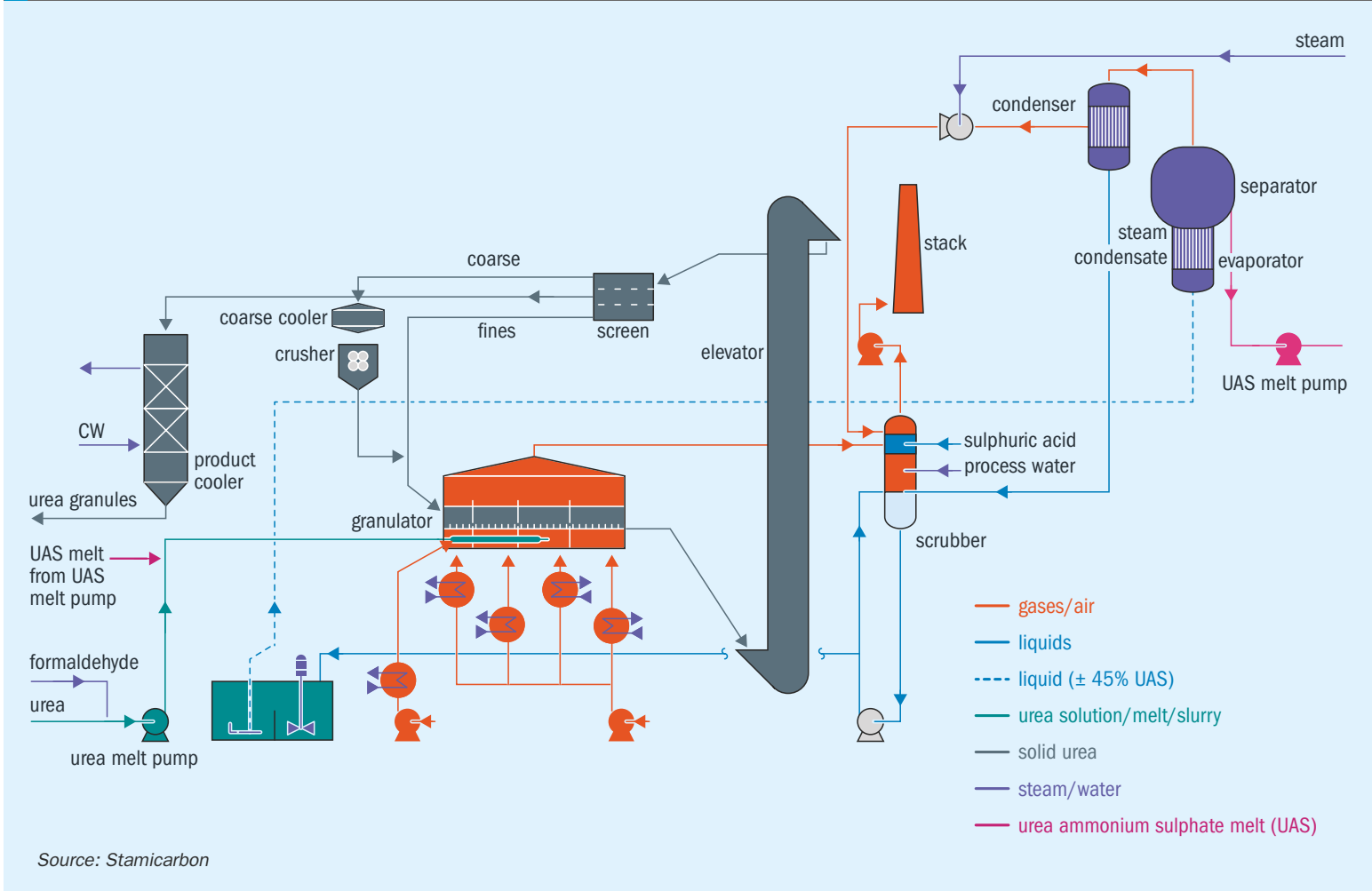
Fig. 3: Process flow diagram of Stamicarbon’s optimised granulation design with an optional recycle evaporator section
