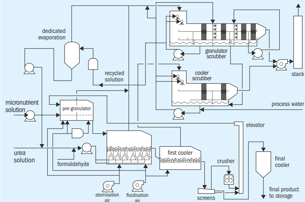
Fig. 3: Pre-granulator technology
