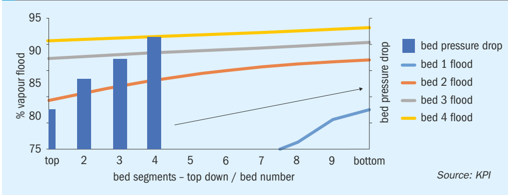
Fig. 5: Stripper bed hydraulics
