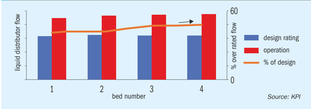
Fig. 6: Stripper liquid distributors – rated vs actual flowrate
