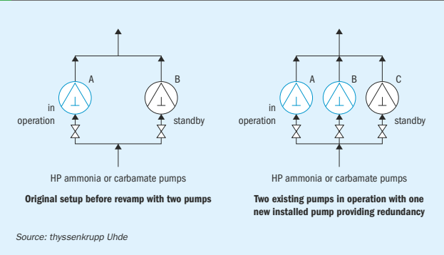
Fig. 6: Standby philosophy for high pressure pumps
