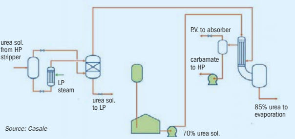
Fig. 8: Addition of a medium-pressure (MP) purification section for revamping CO 2 stripping plants. New equipment shown in white
