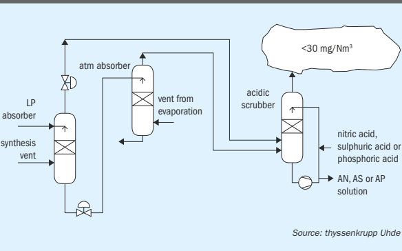
Fig. 3: Ammonia emissions from sources in the melt plant treated with acidic scrubbing
