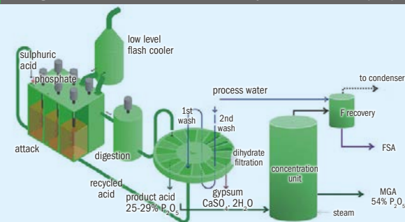
Fig. 1: Simplified scheme for Prayon's di-hydrate (DH) phosphoric acid plant – showing a concentration unit and fluorine recovery as fluorosilicic acid (FSA)
