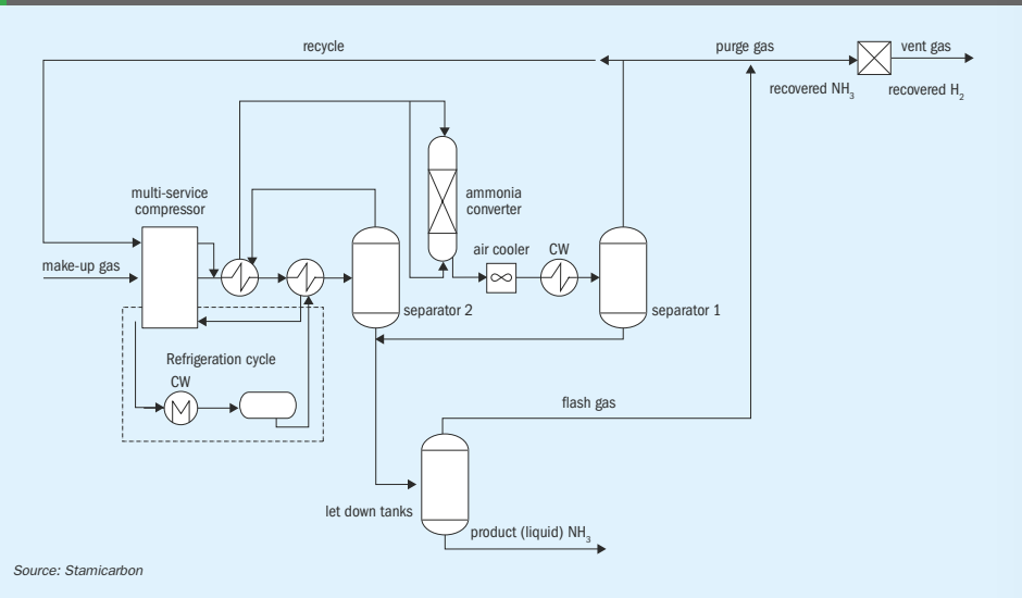
Fig. 2: NX STAMI™ Ammonia High-Pressure Design process diagram
