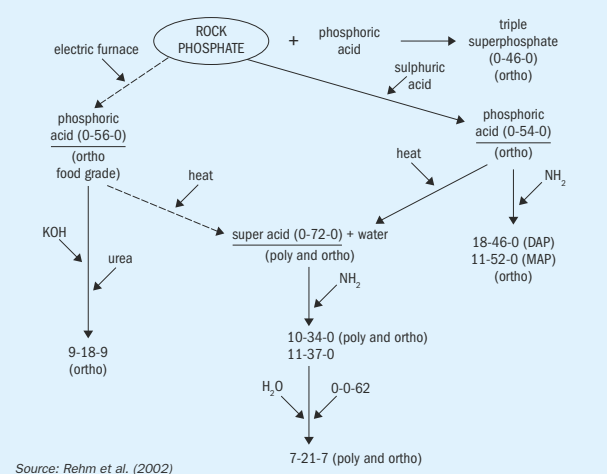
Fig. 3: Schematic of modern phosphate fertilizer production. Rock phosphate (circled) is commonly processed and digested with acid to make the fertilizer products familiar today. Growers can match the phosphate chemistry (ortho or poly) of the fertilizer to their unique crop and soil needs
