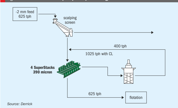
Fig. 3: Customer's revised phosphate processing flowsheet
