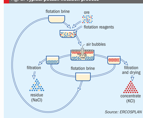
Fig. 1: Typical potash flotation process
