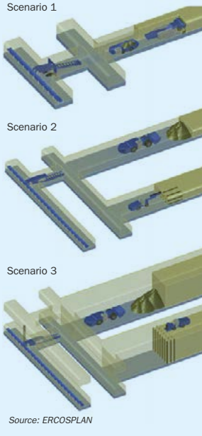
Fig. 3: Three potash mining scenarios: cutting extraction on one mining level (Scenario 1); drilling and blasting on one mining level (Scenario 2); drilling and blasting on two mining levels (Scenario 3).
