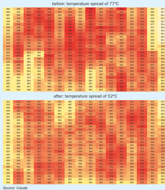
Fig. 2: Temperature heat maps comparing conditions before and after the revamp of the air duct and flue gas tunnel extraction system
