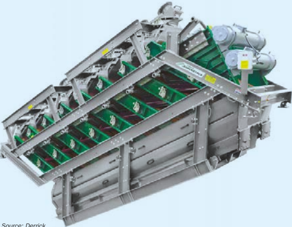
Fig. 1: Derrick® eight-deck SuperStack® fine screening machine for potash
