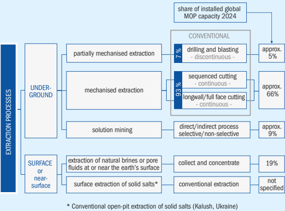
Fig. 1: Overview of the main extraction processes used in muriate of potash (MOP) production, with relative share of 2024 global installed capacities shown
