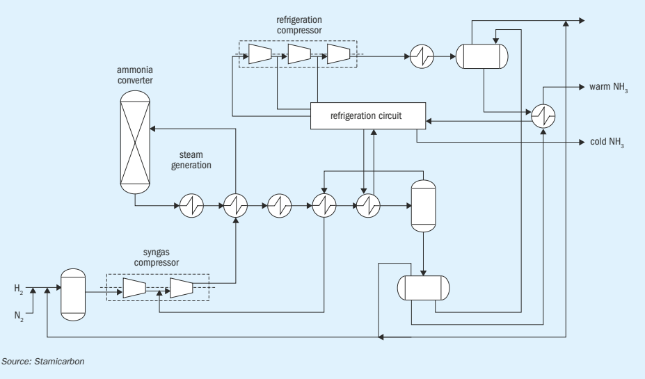
Fig. 1: NX STAMI™ Ammonia Medium-Pressure Design process diagram
