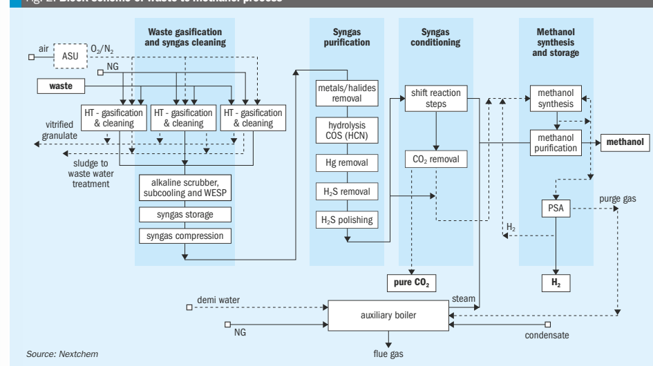
Fig. 2: Block scheme of waste-to-methanol process
