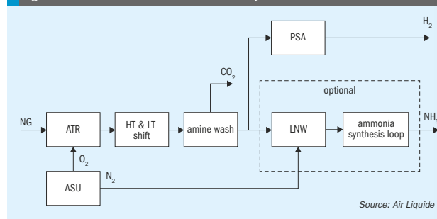
Fig. 3: State-of-the-art amine wash carbon capture solution
