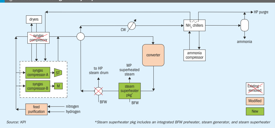
Fig. 3: Case 1: New configuration synloop
