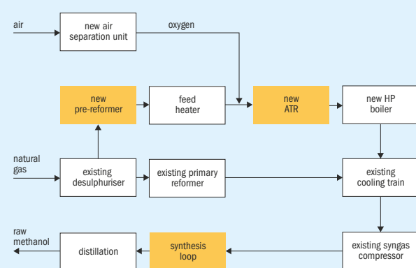
Fig. 4: Upgrade with ATR in parallel with SMR
