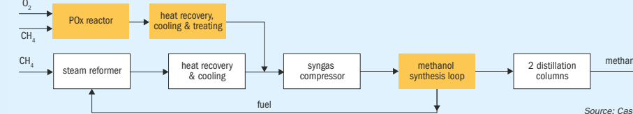
Fig. 7: Revamping strategy through POx
