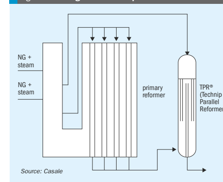
Fig. 3: Reforming section revamp with TPR
