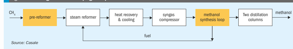
Fig. 1: Reforming section revamping with pre-reformer
