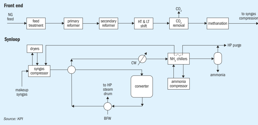
Fig. 1: Case 1: Existing ammonia plant configuration
