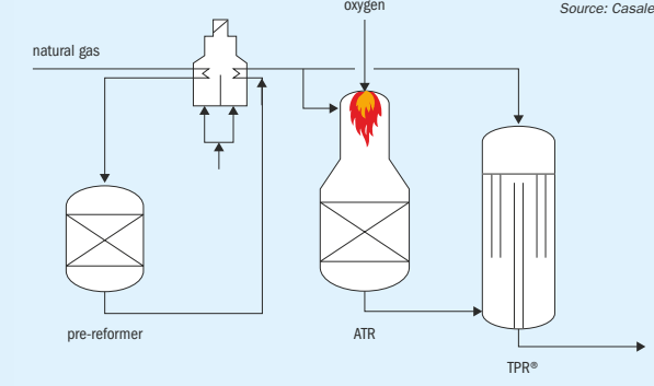
Fig. 7: Revamping strategy through POx
