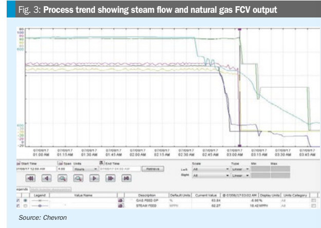
Fig. 3: Process trend showing steam flow and natural gas FCV output
