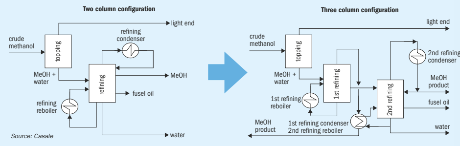
Fig. 11: Distillation revamping concept
