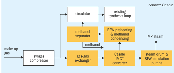
Fig. 10: Synthesis section revamping with OTR
