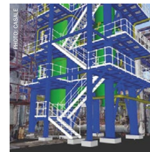
Fig. 8: Syngas generation based on POx (3D model)
