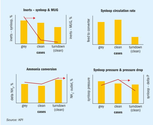
Fig. 2: Case 1: Key variables in synloop
