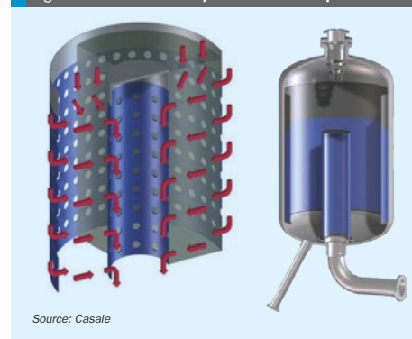
Fig. 2: Casale axial radial pre-reformer concept
