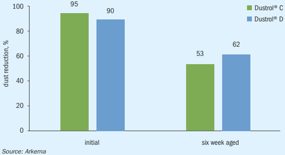
Fig. 2: Modified IFDC dust tower test showing improved dust control behaviour of Dustrol® coated monoammonium phosphate (MAP) fertilizer granules
