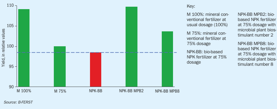
Fig.2: Bio-based fertilizers performance in a 2024 wheat trial in Italy
