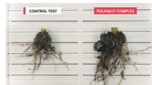
Fig. 2: Comparison of the broccoli root system for control (left) versus Polyhalite Complex (right) treatments.
