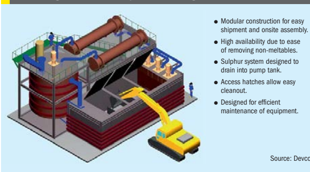
Fig 2: New Wales melter schematic. Rectangular pump tank, cylindrical melter mixing tank and tube-shaped heat exchangers
