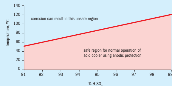
Fig 4: Effect of concentration and temperature for AP cooler
