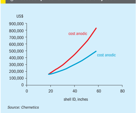
Fig 9: Cost comparison between AP and alloy cooler
