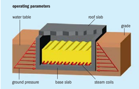
Fig. 1: Typical subsurface reinforced concrete sulphur pit
