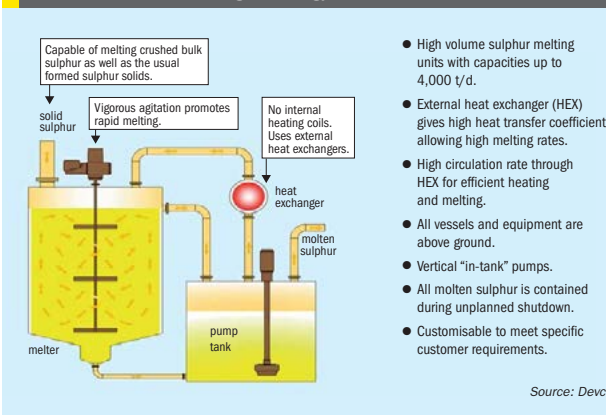
Fig 2: New Wales melter schematic. Rectangular pump tank, cylindrical melter mixing tank and tube-shaped heat exchangers
