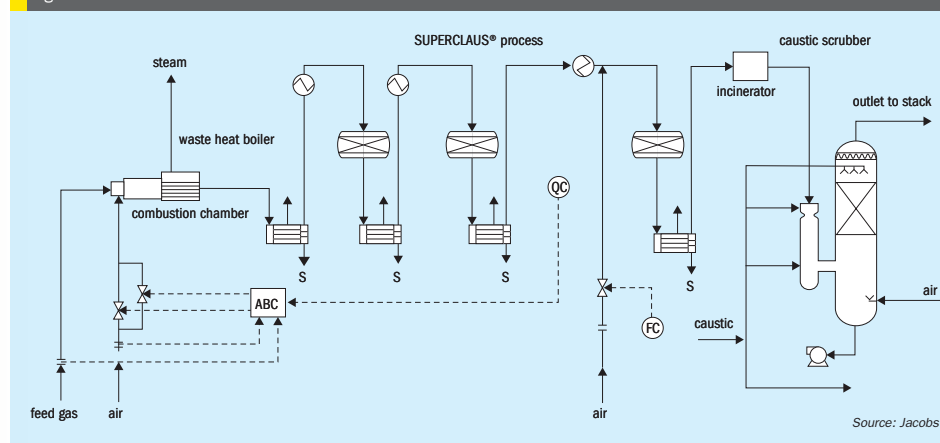
Fig 3: SUPERCLAUS® SRU with caustic scrubber
