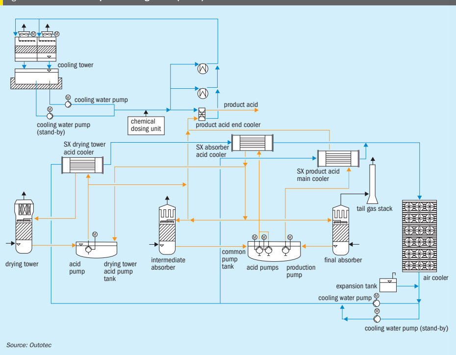
Fig 10: Outotec closed loop acid cooling circuit (model)
