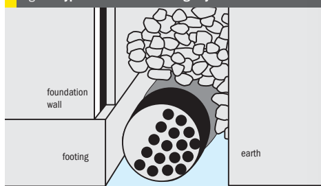
Fig 10: Typical foundation drainage system
