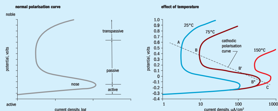
Fig 7: Shifts in polarisation curves
