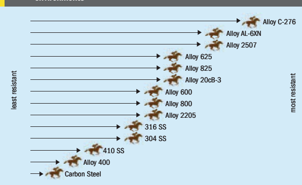
Fig 16: Relative corrosion resistance for test materials in ammonium bisulphide environments 9
