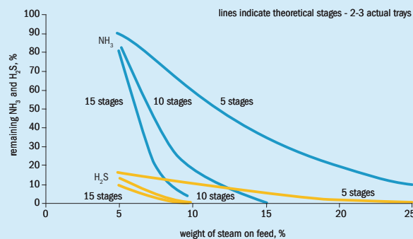
Fig 4: Tray and steam effect on H 2 S and NH 3 removal
