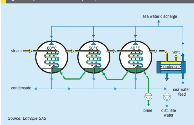
Fig 5: Multiple effect distillation (MED) flow schematic
