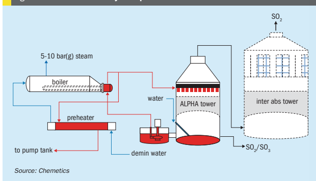
Fig 3: Chemetics ALPHA® system process schematic
