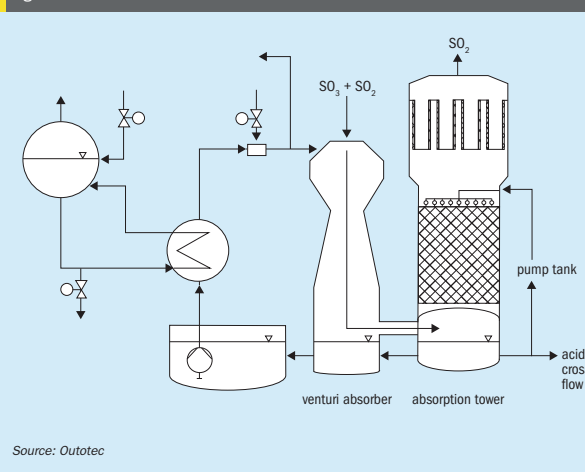
Fig 7: Outotec HEROS solution
