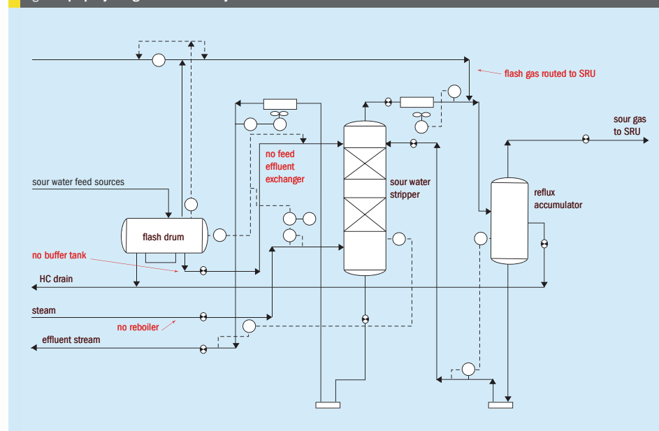
Fig 5: Improperly designed sour water system
