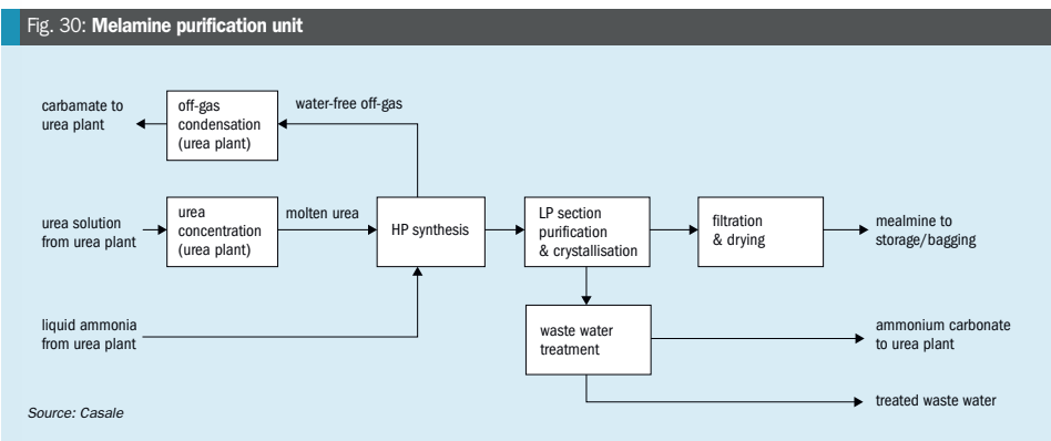
Fig. 30: Melamine purification unit
