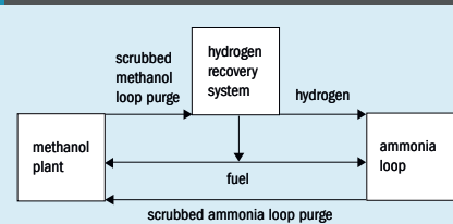
Fig. 11: Connections between methanol plant and ammonia loop
