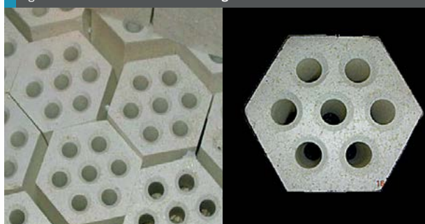
Fig. 9: Condition of KATALCO 94-1ZT target tile after service
