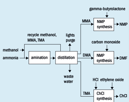
Fig. 19: Methylamines and derivatives
