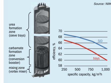
Fig. 9: Efficiency upgrading of the urea synthesis reactor
