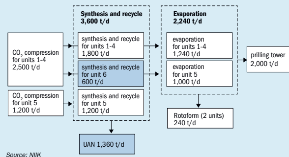
Fig. 8: URECON 2006® urea solution unit
