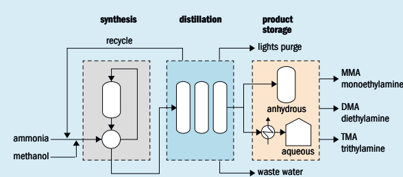
Fig. 20: Methylamines process
