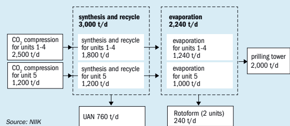
Fig. 7: Urea production after enhancement
