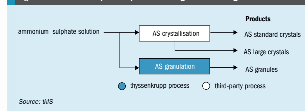
Fig. 32: Ammonium sulphate crystalliser and granulator integration
