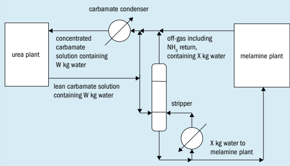
Fig. 23: Eurotecnic integration scheme B – lean carbamate stripping
