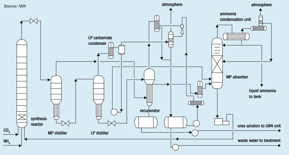
Fig. 8: URECON 2006® urea solution unit
