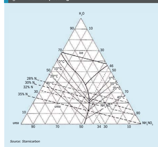
Fig. 3: AN-urea-water phase diagram
