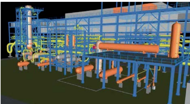
Fig. 26: Casale inert-free NH 3 loop.
