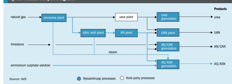
Fig. 33: Fertilizer complex integration
