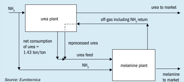
Fig. 22: Eurotecnic integration scheme A – off-gas partial condensation
