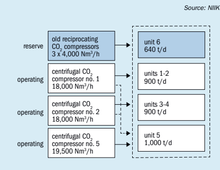
Fig. 10: Distribution of CO 2 compressors by urea plants
