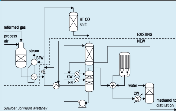
Fig. 15: Saturator-desaturator scheme
