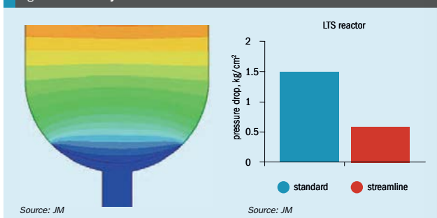
Fig. 11: Case study STREAMLINE flow simulation and results
