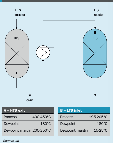
Fig. 13: Possible locations for a Cl-guard in the shift section
