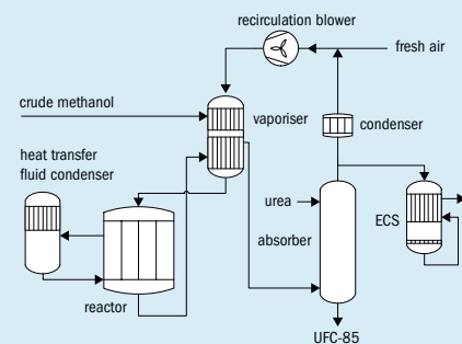
Fig. 17: UFC plant flowsheet
