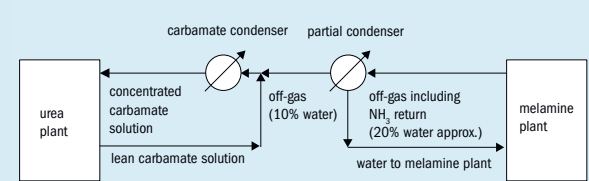
Fig. 22: Eurotecnic integration scheme A – off-gas partial condensation
