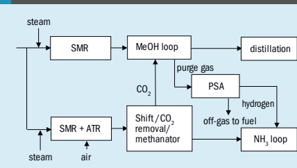
Fig. 14: Separate trains
