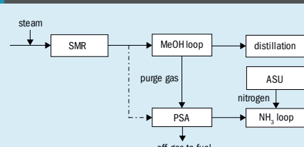
Fig. 12: Single reformer feeding both ammonia and methanol loops
