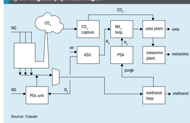
Fig. 25: Integration project block diagram
