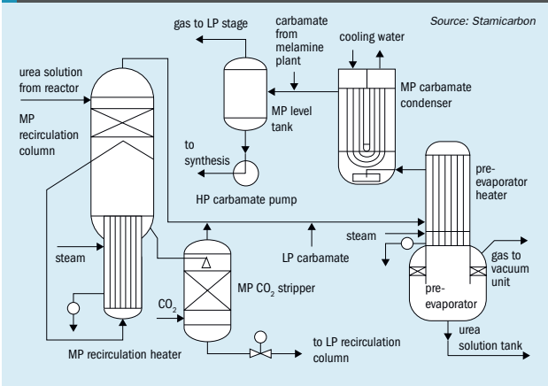
Fig. 4: Urea-melamine coupling with added new MP section
