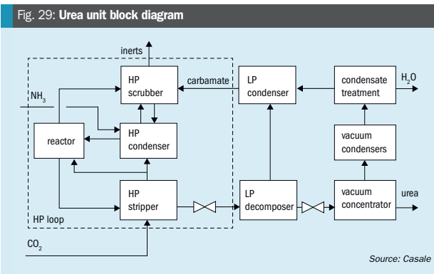
Fig. 29: Urea unit block diagram
