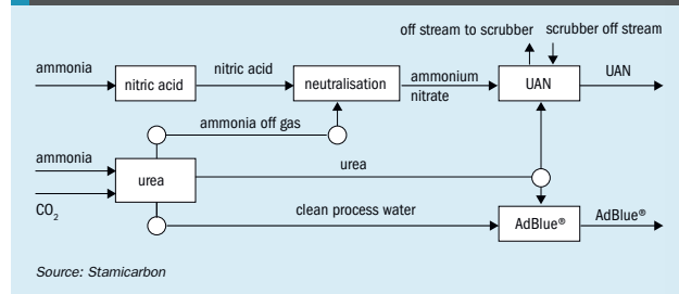
Fig. 5: Stamicarbon's fully integrated UAN plant
