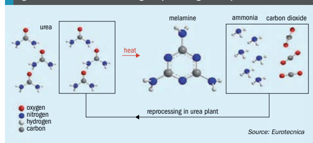
Fig. 1: Melamine reaction with off-gas reprocessing in urea plant
