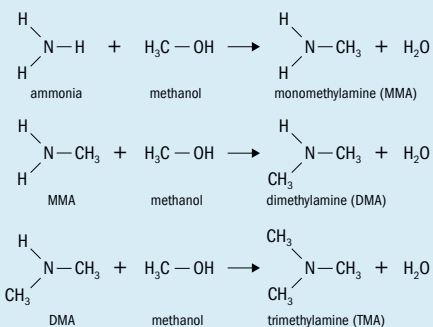
Fig. 18: Methylamines chemistry
