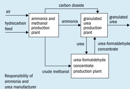
Fig. 16: JM's FORMOX integrated UFC process
