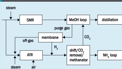
Fig. 13: Johnson Matthey integrated flowsheet
