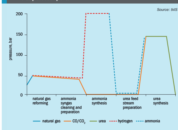
Fig 2: Ammonia and CO 2 pressure variations in current ammonia/urea production plants
