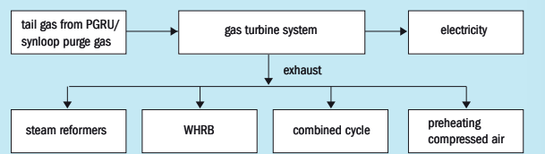
Fig 3: Gas turbine schematic for ammonia plant
