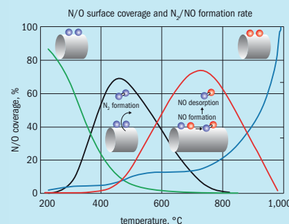
Fig 6: Simulated correlation of N/O surface coverage and relative N_2/NO formation rate
