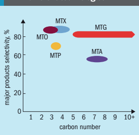
Fig 1: Major product selectivity versus carbon number for different technologies
