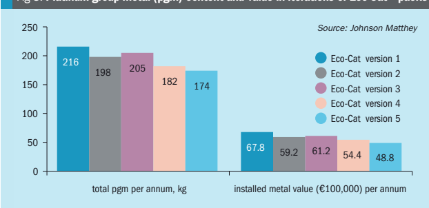
Fig 9: Platinum group metal (pgm) losses in iterations of Eco-Cat™ packs
