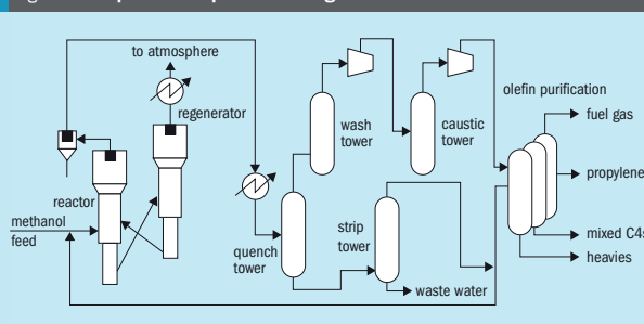
Fig 4: CMTX process simplified flow diagram
