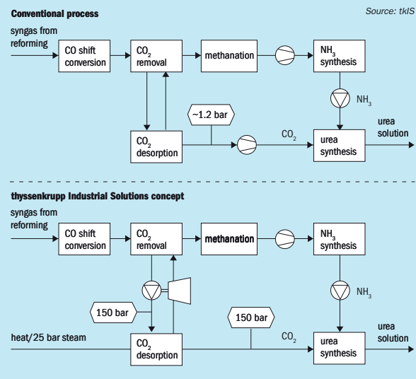
Fig 3: Comparison of conventional scheme and alternative thyssenkrupp Industrial Solutions concept
