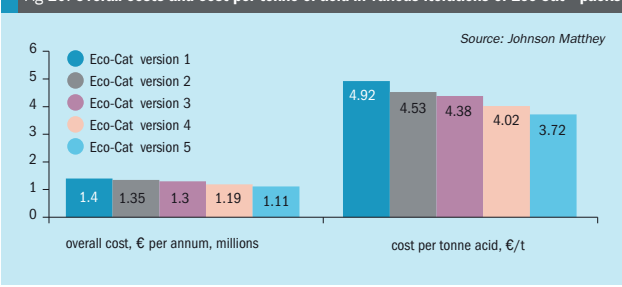
Fig 10: Overall costs and cost per tonne of acid in various iterations of Eco-Cat™ packs
