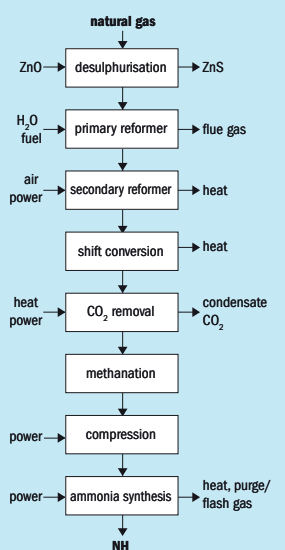
Fig 2: Block diagram of ammonia manufacturing process
