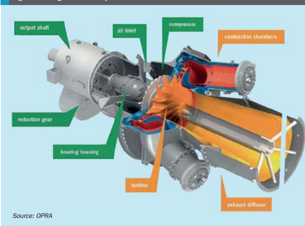
Fig 1: OP16 gas turbine system
