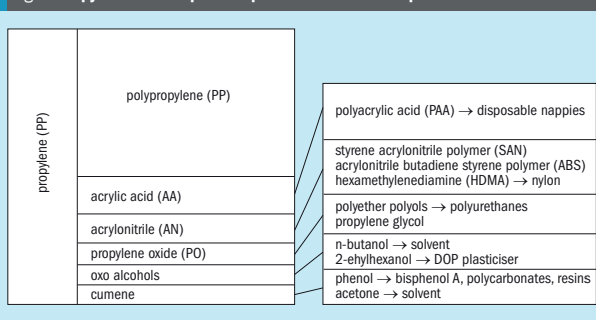
Fig 2: Propylene consumption to produce downstream products
