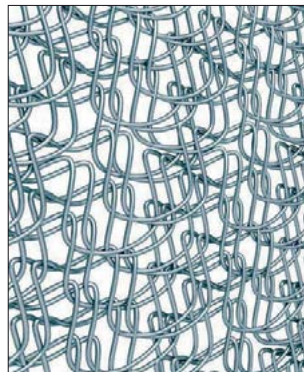
SAFINA knitted catalyst gauze structure.
