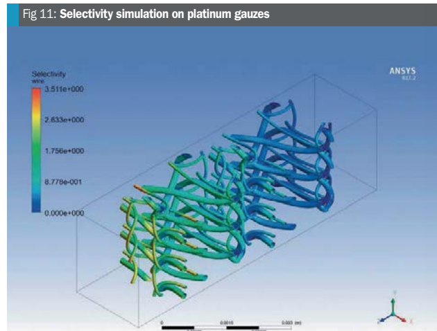
Fig 11: Selectivity simulation on platinum gauzes
