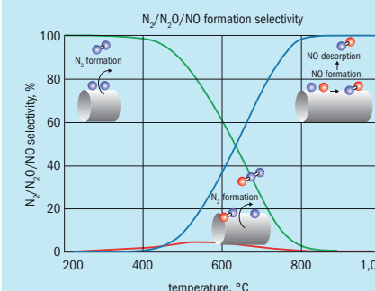
Fig 7: Simulated correlation of N_2/N_2O/NO selectivity and gauze temperature
