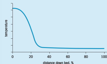
Fig 2a: Typical bed temp. profile for natural gas pre-reforming
