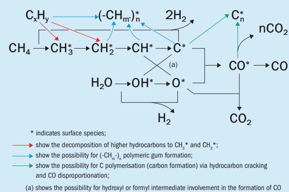
Fig 3: A possible reaction mechanism for steam reforming
