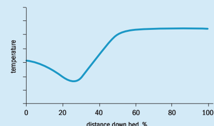
Fig 2b: Typical bed temp. profile for naphtha pre-reforming
