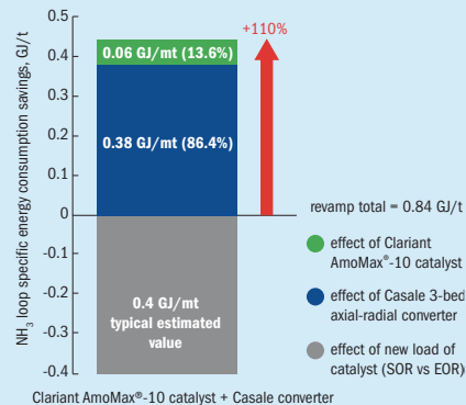
Fig 14: NH 3 synthesis loop specific energy consumption savings
