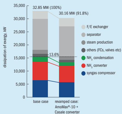
Fig 13: Exergy analysis for the base case vs revamped case: dissipation of exergy
