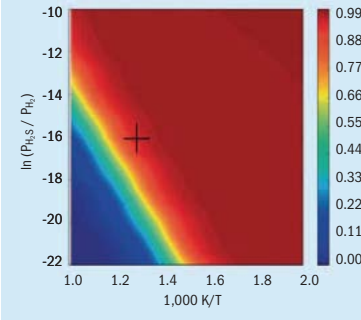
Fig 11: Calculated isostere of sulphur
