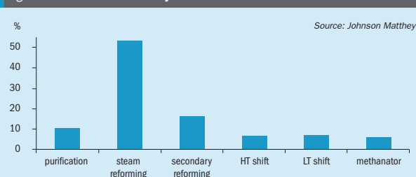
Fig 1: Ammonia front end catalyst \Delta P
