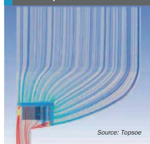
Fig 20: CFD model of original elephant stool
