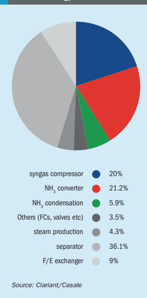
Fig 12: Results of the exergy balance for the base case: distribution of exergy losses
