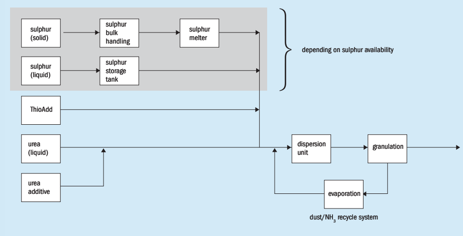
Fig 3: Basic flow sheet for a sulphur-enhanced urea granulation plant
