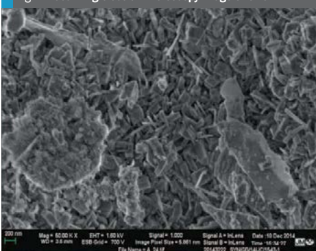
Fig 14: Scanning electron microscopy image of CRG LH
