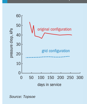
Fig 22: Pressure drop of LTS reactor (new grid configuration: 10 month service life)
