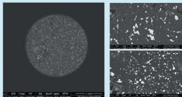
Fig 2: Scanning electron microscopy of a 13% ES Urea-ES sample
