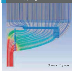
Fig 21: CFD model of catalyst support grid
