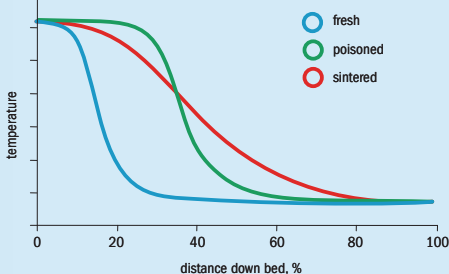
Fig 6: Natural gas bed temperature profile
