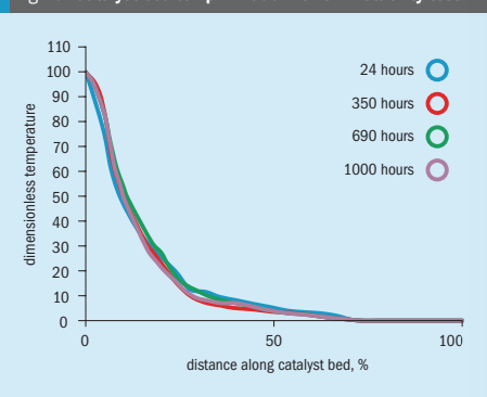
Fig 15: Catalyst bed temp in 1000 h CRG LH stability test
