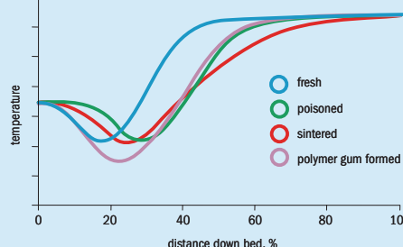
Fig 7: Naphtha bed temperature profile
