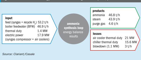
Fig 10: Results of the energy balance case: diagram of inputs, products and losses
