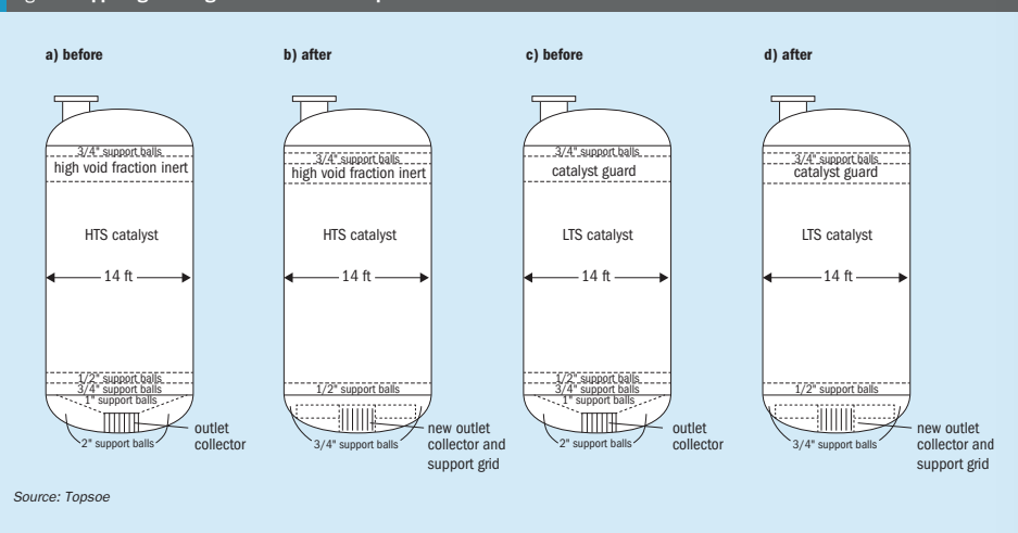
Fig 17: Support grid design before and after replacement
