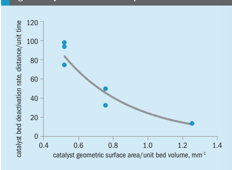
Fig 9: Catalyst surface area vs sulphur deactivation rates
