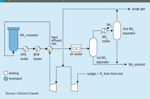
Fig 8: Simplified process flow diagram of the ammonia synthesis loop
