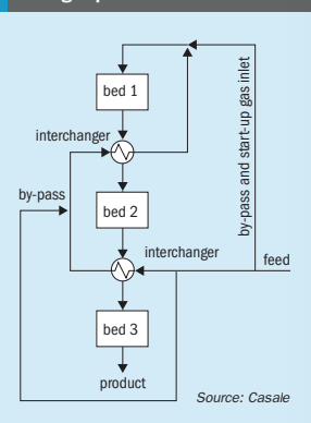
Fig 9: Casale 3-bed-2-ICH converter gas path
