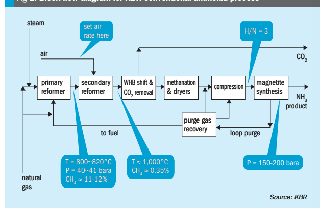
Fig 1: Block flow diagram for KBR conventional ammonia process
