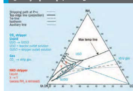
Fig 1: NH 3 -CO 2 -urea-H 2 O phase diagram
