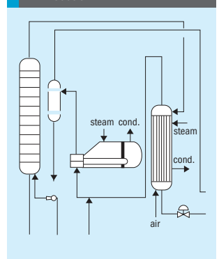
Fig 8: Layout of Saipem synthesis section
