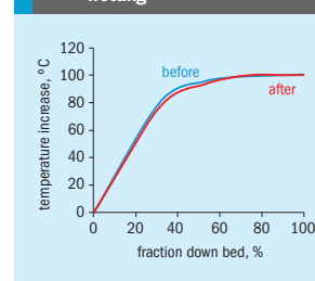
Fig 6: Exotherm before and after wetting
