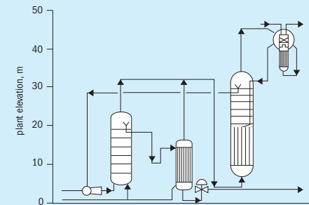
Fig 4: THESES synthesis layout
