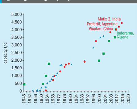
Fig 7: Largest design capacity awarded in time
