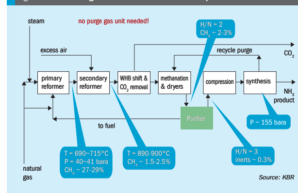
Fig 3: Sketch of KBR Purifier™
