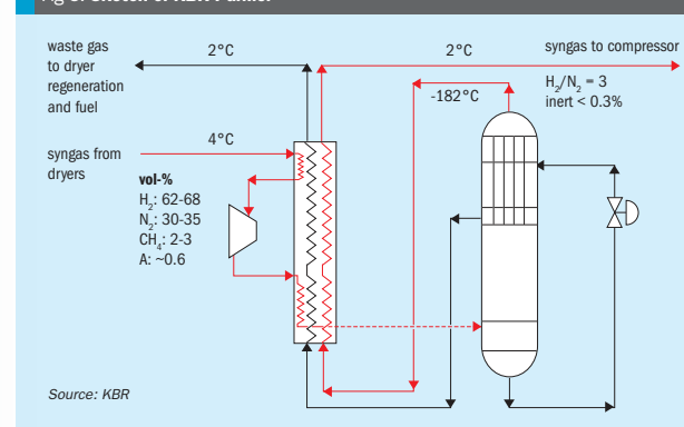
Fig 3: Sketch of KBR Purifier™
