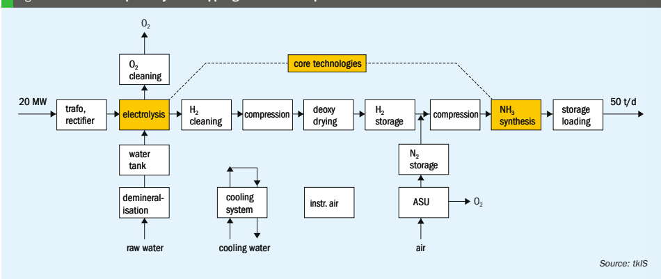
Fig. 5: Process concept of thyssenkrupp's green ammonia production
