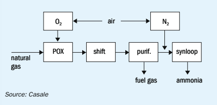
Fig. 9: Casale A60™ ammonia plant block flow diagram
