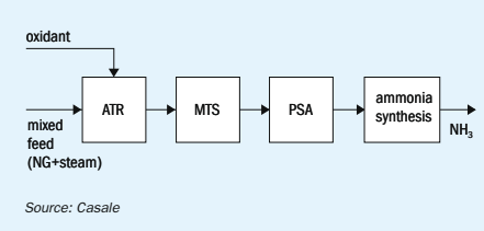
Fig. 10: Casale A600™ ammonia plant block flow diagram
