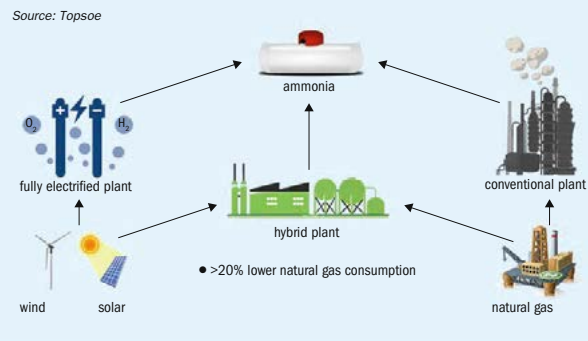
Fig. 1: The hybrid plant solution
