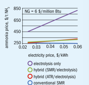
Fig. 2: Ammonia production price versus electricity cost
