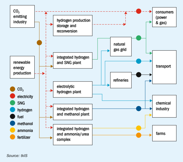
Fig. 4: Hydrogen value chains by thyssenkrupp
