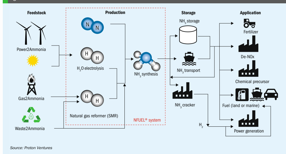
Fig. 7: NFUEL® overview
