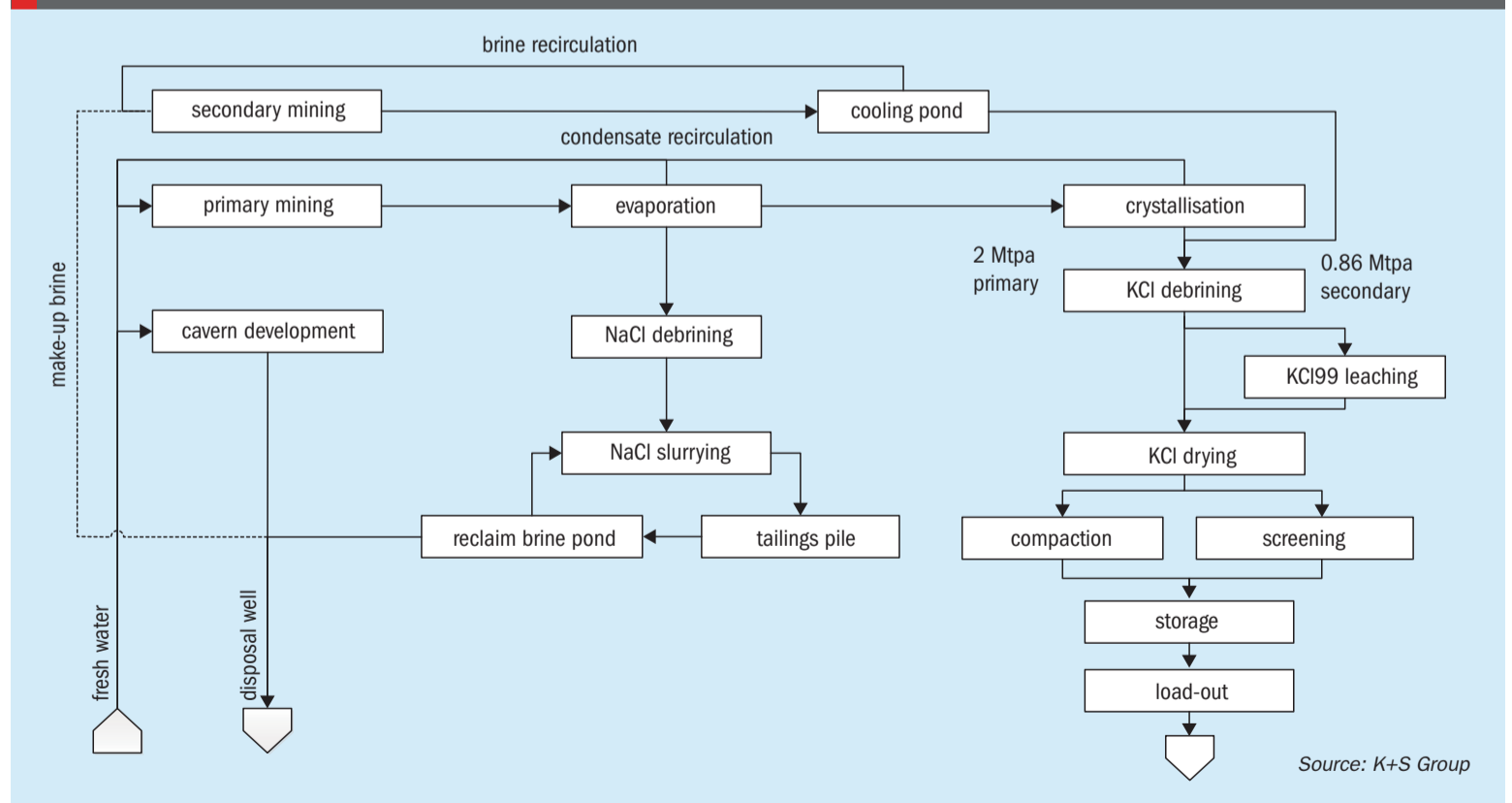
Fig 1: Legacy project process flowsheet
