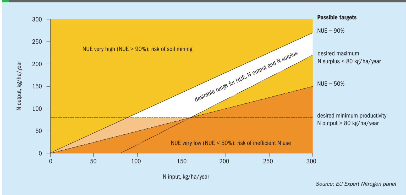
Fig 2: Nitrogen input-output diagram with possible targets for NUE, N output and surplus
