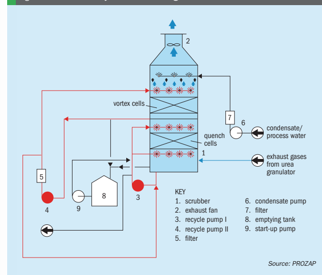
Fig 4: Scrubber cutaway view with six stages indicated
