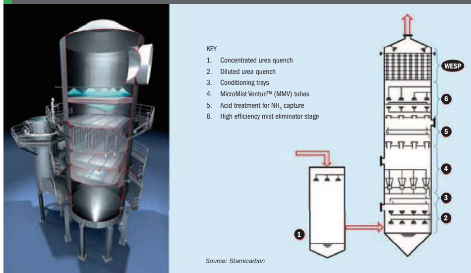
Fig 3: Scrubber cutaway view with six stages indicated
