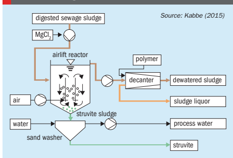
Fig 2: The AirPrex struvite crystallisation process from sludge
