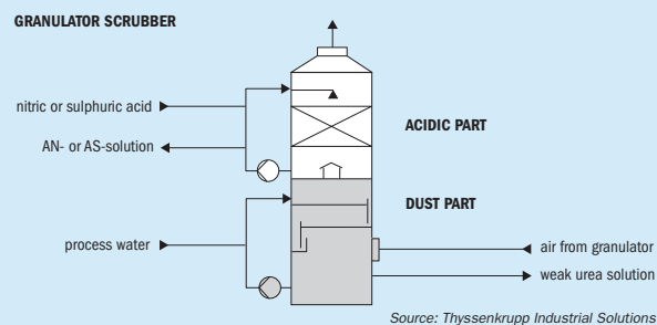
Fig 1: Typical two-stage granulation plant scrubber
