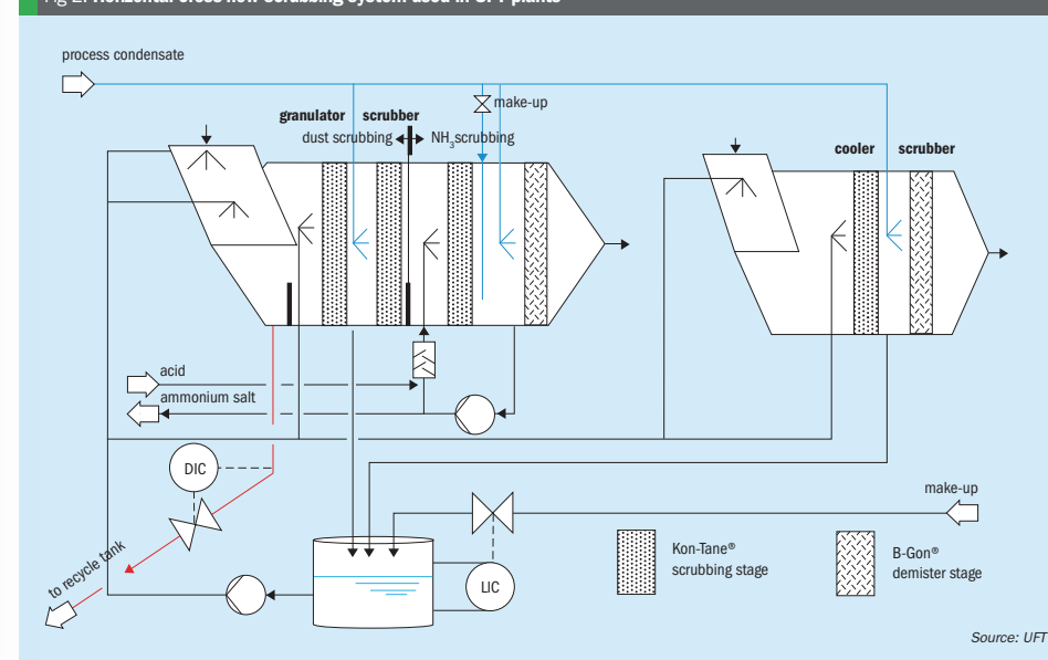
Fig 2: Horizontal cross-flow scrubbing system used in UFT plants
