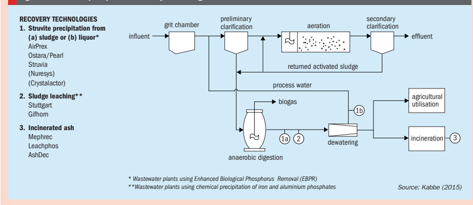
Fig 4: Wastewater phosphorus recovery technologies
