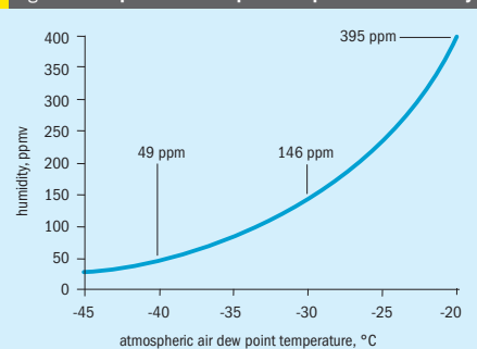
Fig. 5: Atmospheric air dew point temperature vs humidity
