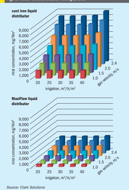
Fig. 8: Mist concentration comparison
