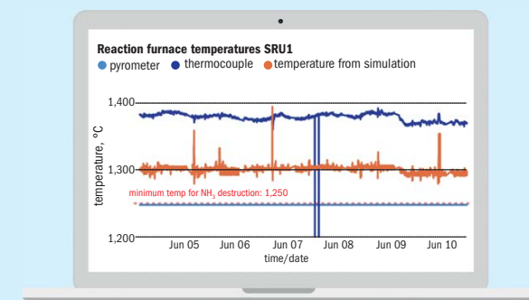
Fig. 3: Combustion chamber temperature measured by the pyrometer, thermocouple and calculated via simulations
