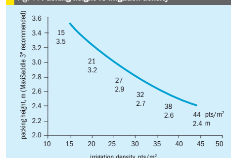
Fig. 7: Packing height vs irrigation density
