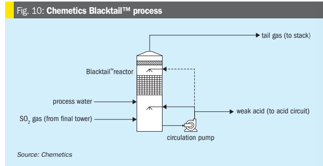
Fig. 10: Chemetics Blacktail™ process
