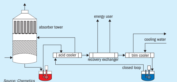
Fig. 6: Closed loop heat recovery system to produce hot water
