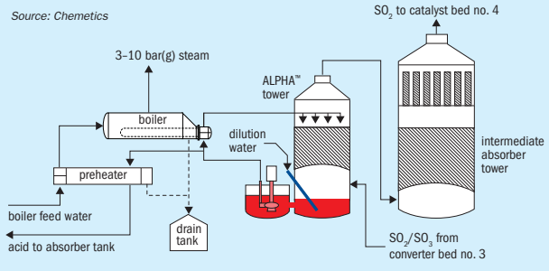
Fig. 7: Chemetics ALPHA™ system
