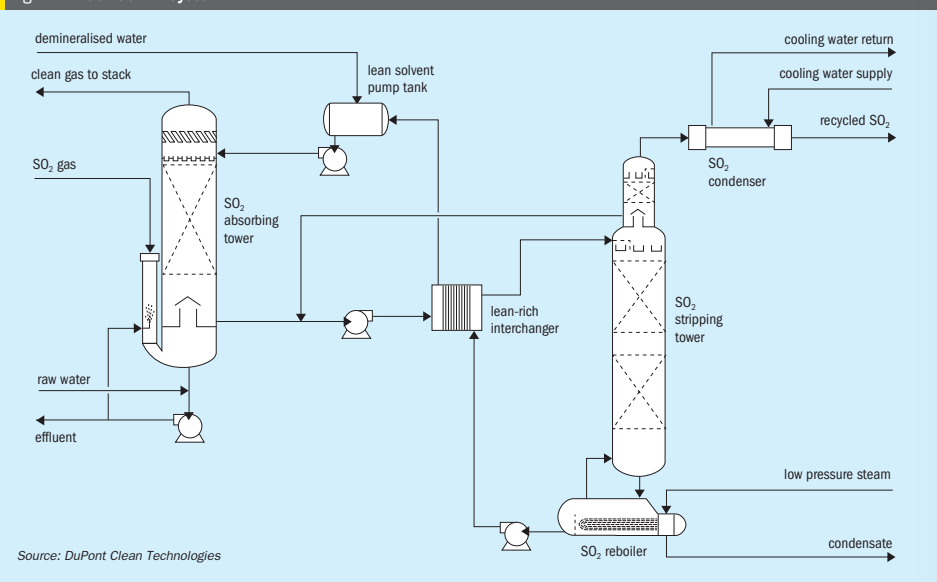
Fig. 2: MECS® SolvR® system
