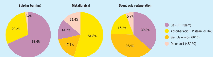
Fig. 5: Typical recoverable energy profile for sulphuric acid plants
