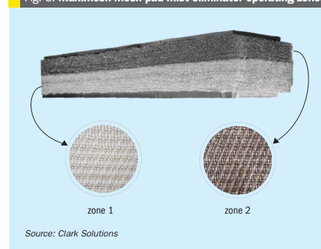
Fig. 3: Maximesh mesh pad mist eliminator operating zones
