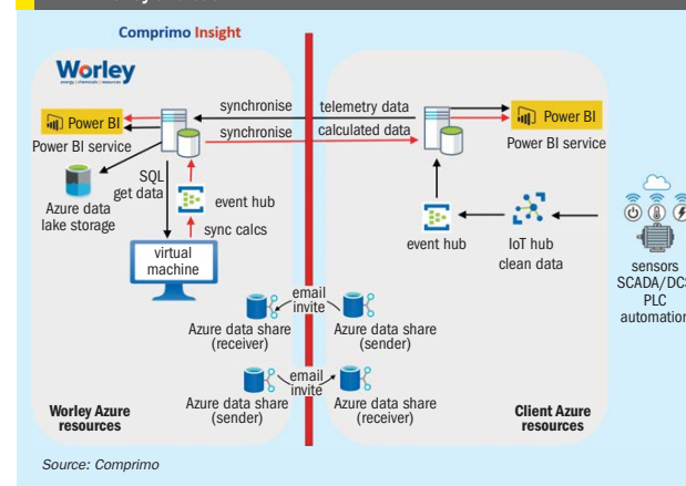
Fig. 1: Schematic representation of the data transfer model from customer to Worley and back
