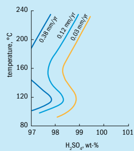
Fig. 12: 310S stainless steel isocorrosion lines
