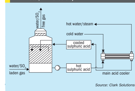
Fig. 3: SAFEHX® acid cooling (heat transferred to cooling water, BFW or others)
