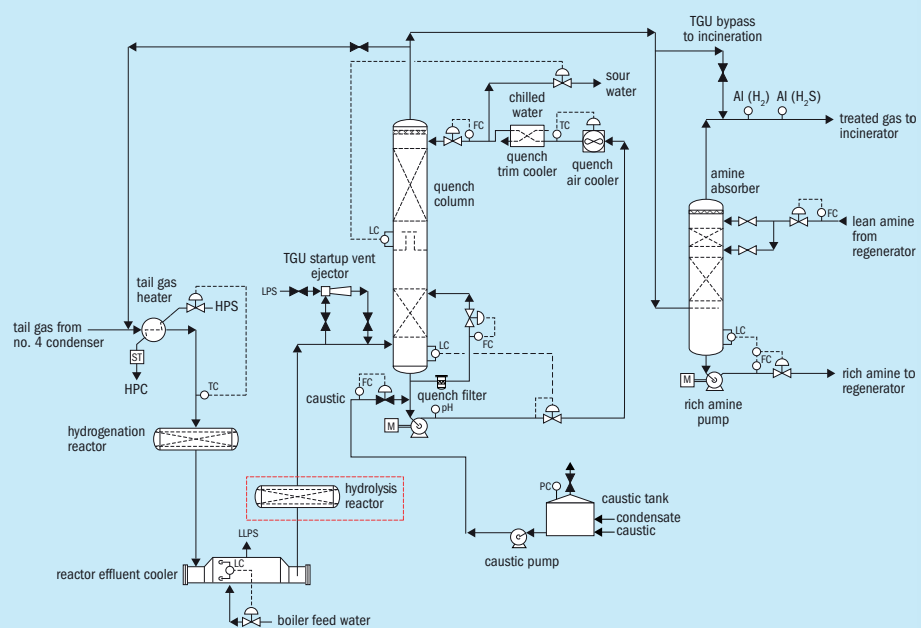
Fig. 5: RATE tail gas scheme
