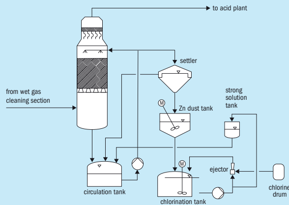
Fig. 4: Metso Outotec's B-N mercury removal process
