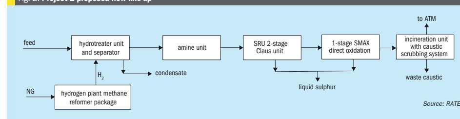
Fig. 2: Project 2 proposed new line-up
