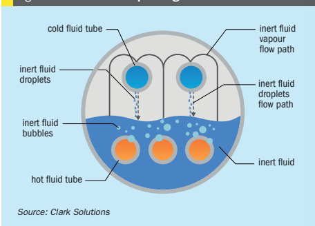
Fig. 1: Basic SAFEHX® operating scheme
