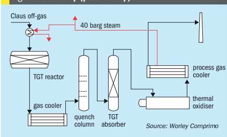
Fig. 2: New line-up (post revamp)
