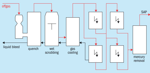
Fig. 1: Wet gas cleaning system
