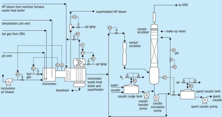
Fig. 6: Tail gas incineration with caustic scrubber
