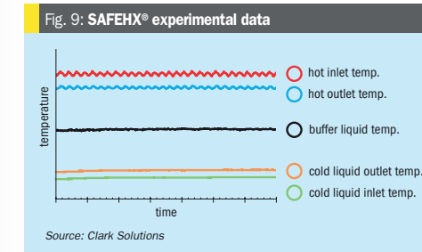
Fig. 9: SAFEHX experimental data
