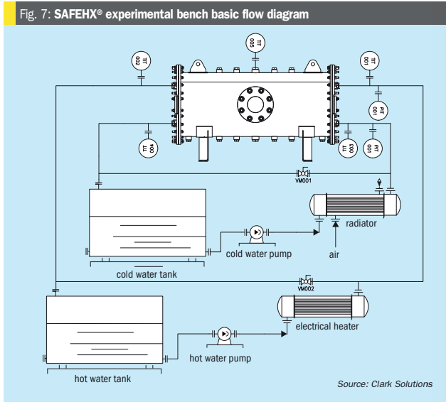
Fig. 7: SAFEHX experimental bench basic flow diagram
