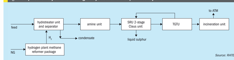
Fig. 1: Simplified refinery scheme showing the hydrotreater and sulphur recovery unit
