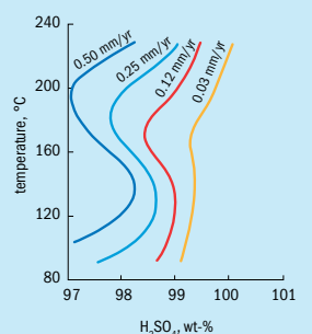
Fig. 11: 304L stainless steel isocorrosion lines
