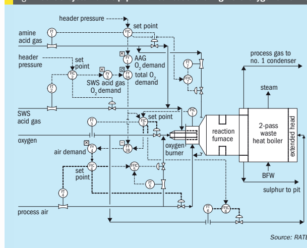
Fig. 4: Control system and equipment modifications for high-level oxygen enrichment
