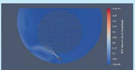
Fig. 8a: BFW inlet distributor improperly installed, rotated 45°
