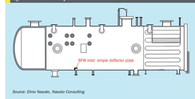
Fig. 7: WHB rudimentary boiler feedwater inlet
