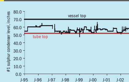
Fig. 12: First condenser - historical water level
