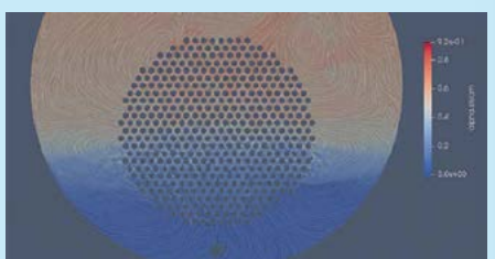
Fig. 8b: BFW inlet distributor properly installed
