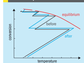
Fig. 1: Temperature optimisation of a four-pass converter
