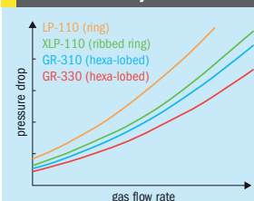
Fig. 2: Relative pressure drop for clean catalyst
