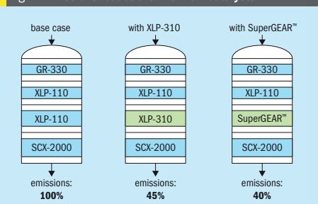
Fig. 4: Emissions reductions with new catalysts
