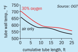
Fig. 2: Tube wall temp. in WHB pass 1
