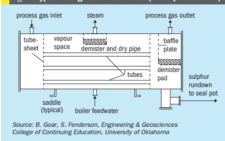
Fig. 4: Typical straight shell condenser (Claus process SRU)
