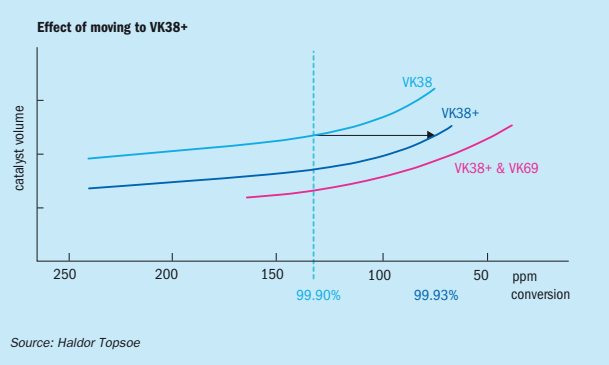
Fig. 1: Lower emission with the same volume
