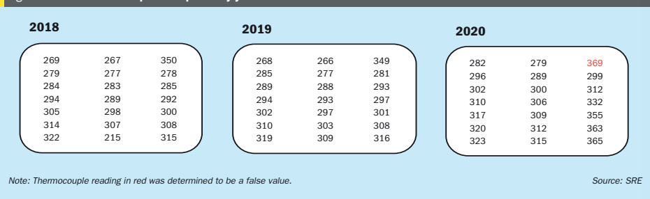
Fig. 1: First converter temperature profile by year
