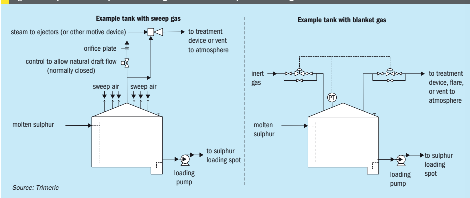
Fig. 5: Example molten sulphur tank configurations with sweep air and inert gas blanket
