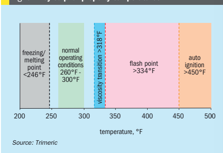
Fig. 3: Key sulphur property temperatures
