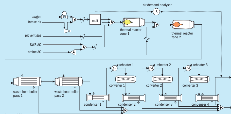
Fig. 1: SRU configuration
