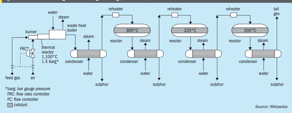
Fig. 1: Schematic flow diagram of a straight-through, 3 reactor, Claus SRU
