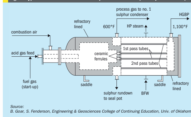
Fig. 2: Typical thermal reactor and two pass kettle WHB (Claus process SRU)
