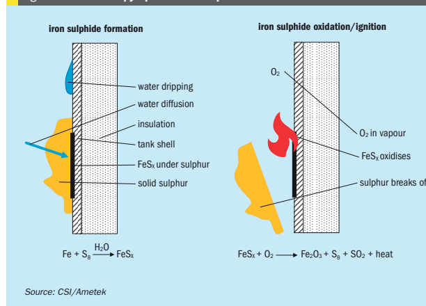
Fig. 4: Formation of pyrophoric iron sulphide
