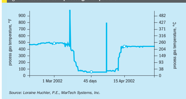
Fig. 13: Last condenser – process gas temperature
