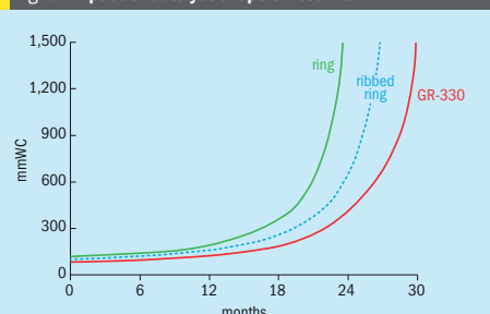
Fig. 3: Impact of catalyst shape on bed life
