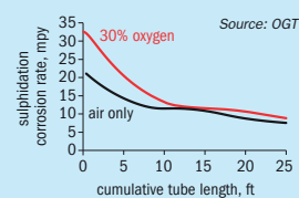
Fig. 3: Corrosion rates in WHB pass 1
