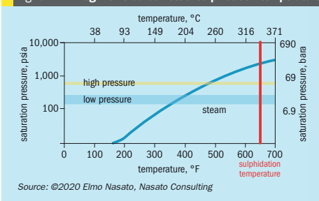
Fig. 5: WHB regime vs carbon steel sulphidation temperature
