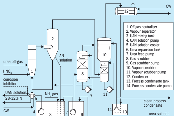
Fig. 8: uhde® urea off-gas neutralisation (simplified scheme)
