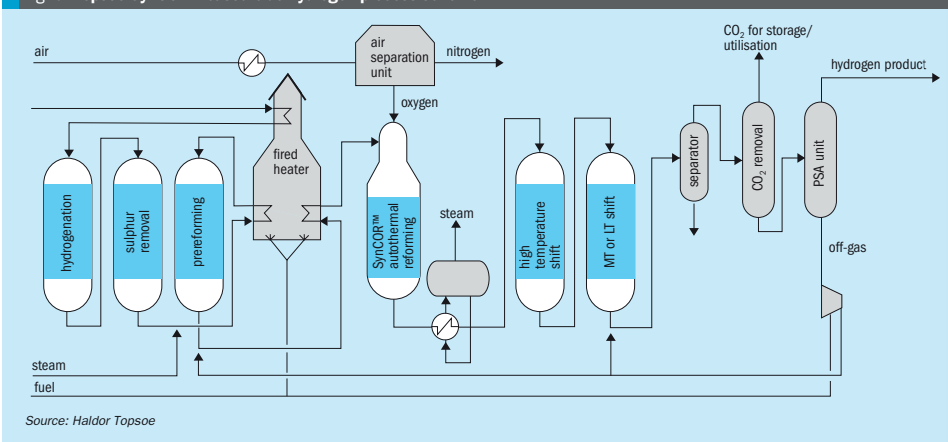
Fig. 6: Topsoe SynCOR™ based blue hydrogen process scheme
