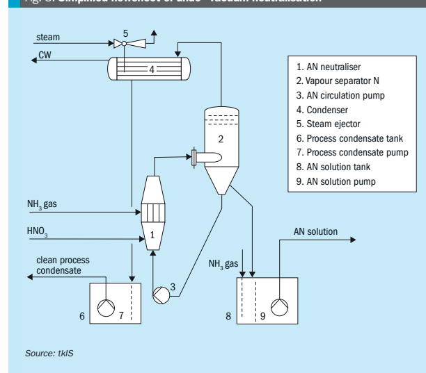
Fig. 3: Simplified flowsheet of uhde® vacuum neutralisation
