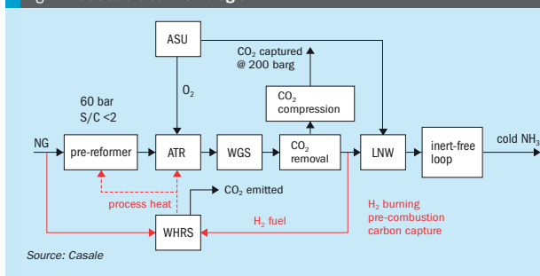
Fig. 7: A6000CC block flow diagram
