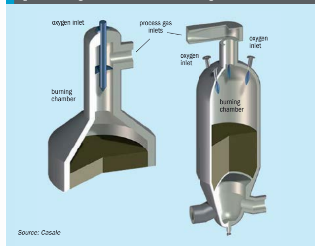
Fig. 9: Casale single-burner and multi-burner ATR design
