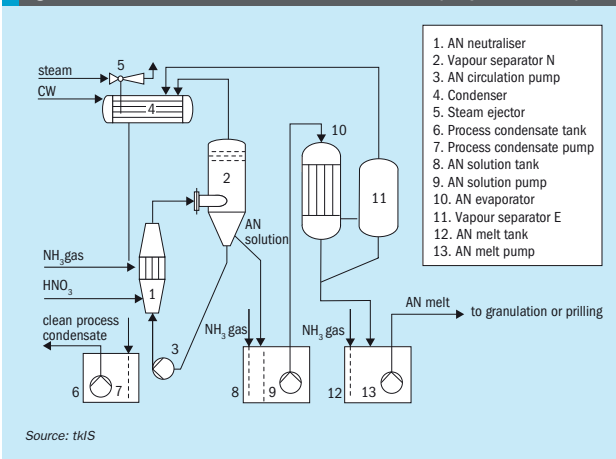
Fig. 6: combined uhde® neutralisation and concentration (simplified scheme)
