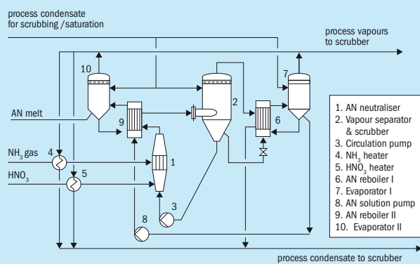
Fig. 7: uhde® AN pressure neutralisation and concentration (simplified scheme)
