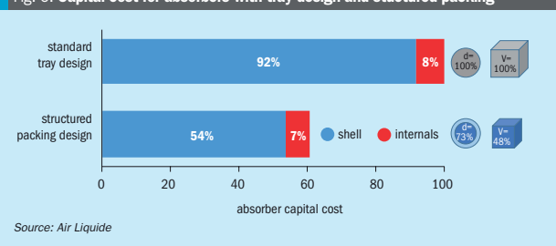
Fig. 6: Capital cost for absorbers with tray design and structured packing
