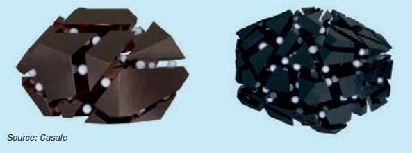
Fig. 10: Differences between AmoMax-Casale and standard iron catalyst
