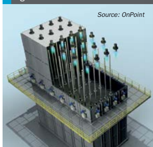
Fig. 3: ZoloSCAN installation
