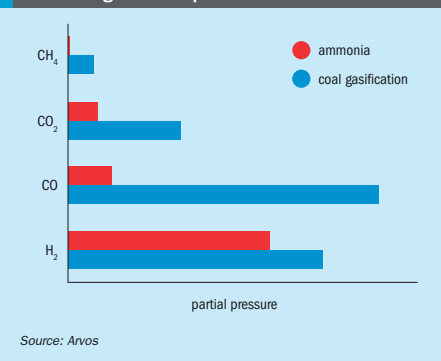
Fig. 3: Comparison of gas partial pressures in ammonia vs coal gasification plants
