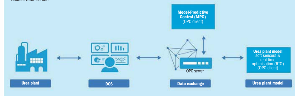
Fig. 1: Architecture of the Stami Digital Plant Optimiser system
