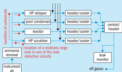
Fig. 1: Leak in pressurised leak detection system
