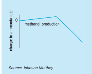
Fig. 3: Effect of production rate of methanol synthesis retrofit installed downstream of CO 2 removal stage on potential ammonia production rate
