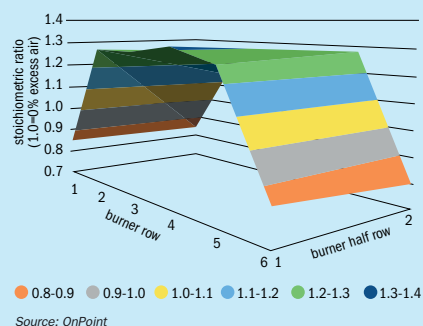
Fig. 6: Burner stoichiometry map before Ember tuning
