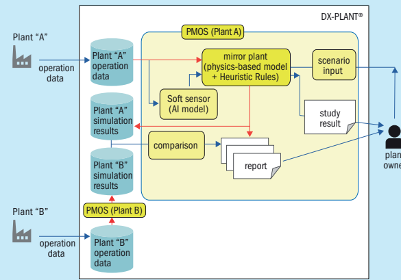
Fig. 14: Overall configuration of PMOS™
