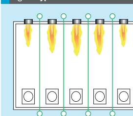
Fig. 2: Typical down-fired reformer
