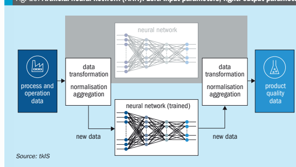
Fig. 19: Artificial neural network (ANN): Left: Input parameters; right: output parameters
