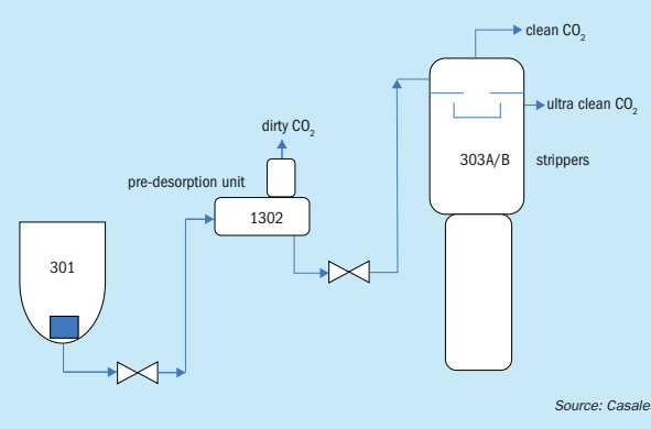
Fig. 7: Simplified scheme between items 301 and 303A/B
