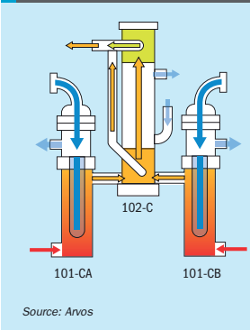
Fig. 1: Typical arrangement of vertical primary and secondary PGCs
