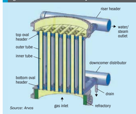
Fig. 2: Schmidt'sche® double tube system
