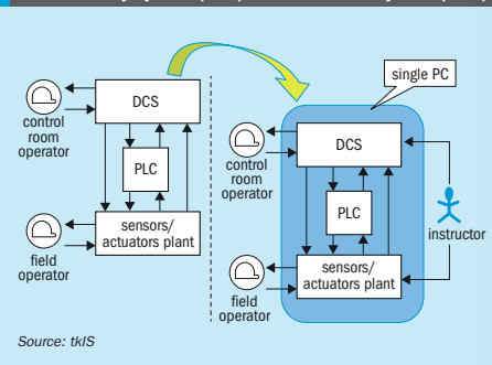
Fig. 22: Schematic picture of the real plant (left side) and simulated plant (right side) including the plant, the safety system (PLC) and the control system (DCS)
