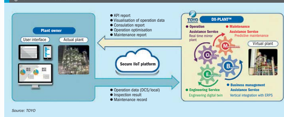
Fig. 10: DX-PLANT® architecture
