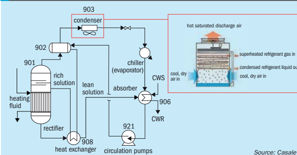
Fig. 1: Typical AARP revamping approach
