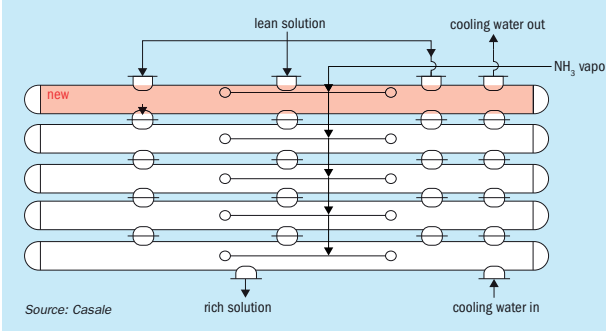
Fig. 2: Additional CW exchangers providing greater surface area in ammonia absorber
