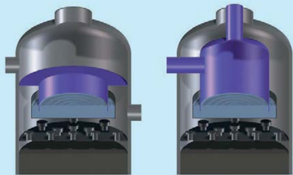
Fig. 6: Internal separation device for new and revamped tower
