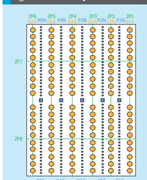
Fig. 5: ZoloSCAN layout
