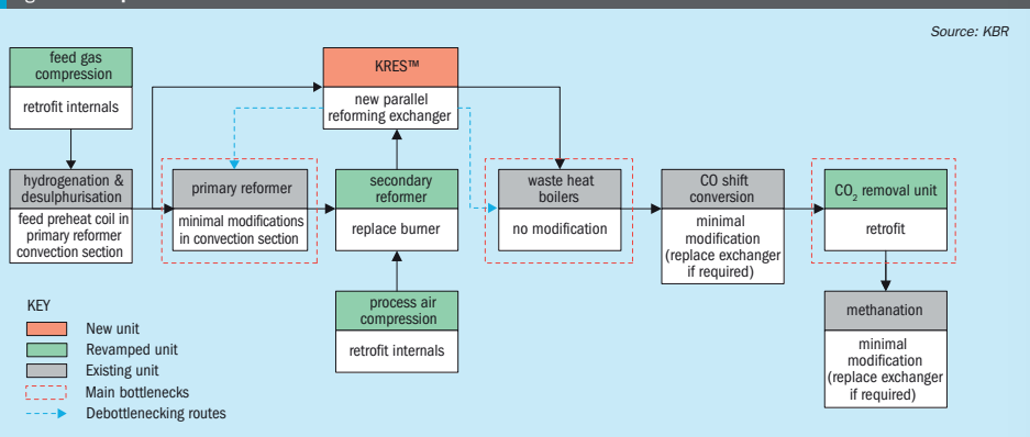
Fig. 1: Revamp scheme of front end
