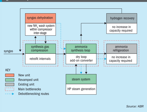
Fig. 3: Revamp scheme of back end
