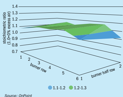
Fig. 8: Burner stoichiometry map after Ember tuning
